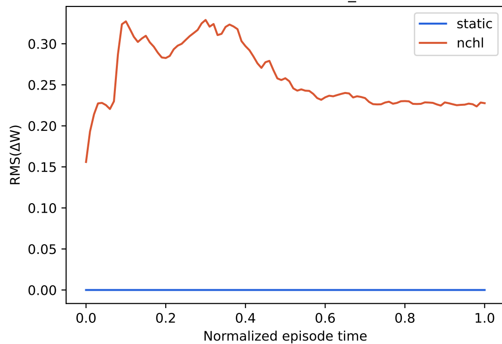
Thrower-v0 / thrower_arm
