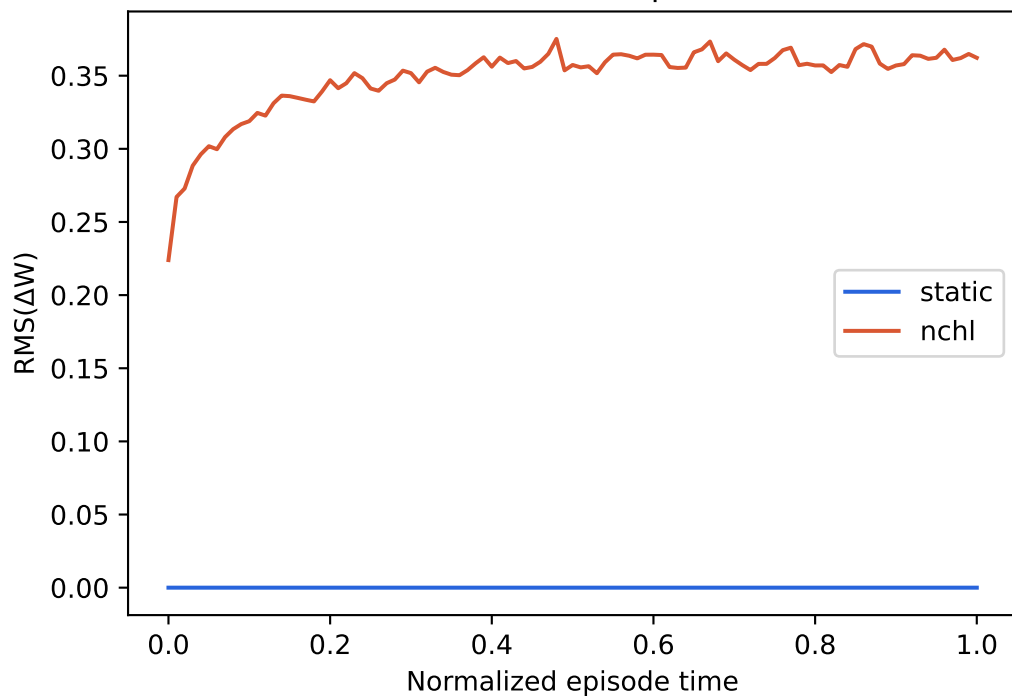
Walker-v0 / biped
