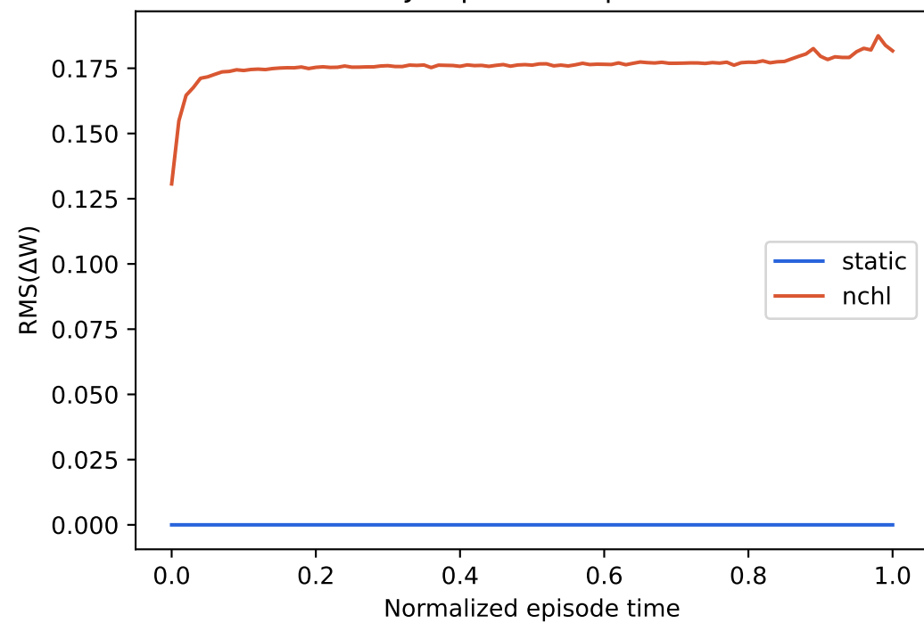
Thrower-v0 / thrower_arm
