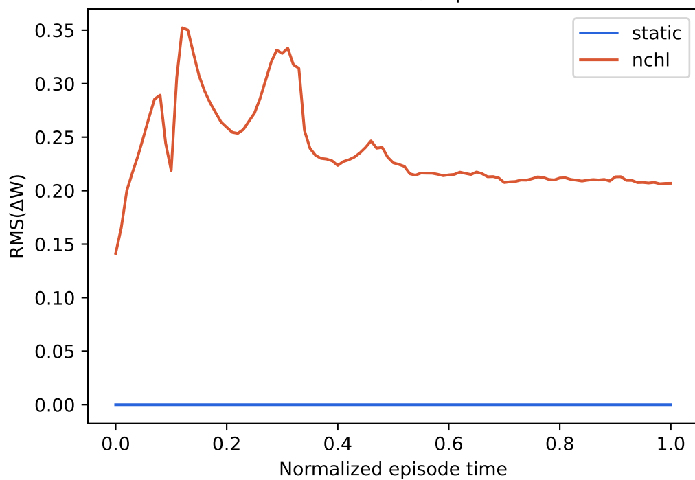
Walker-v0 / biped
