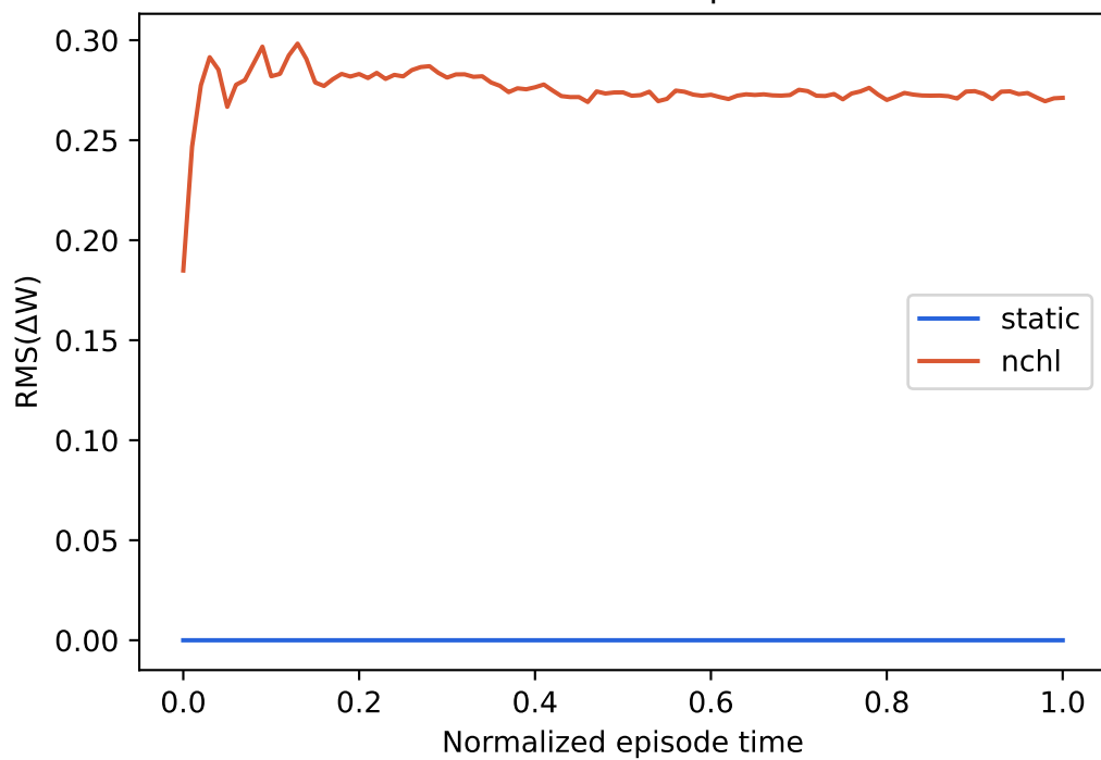
Thrower-v0 / biped
