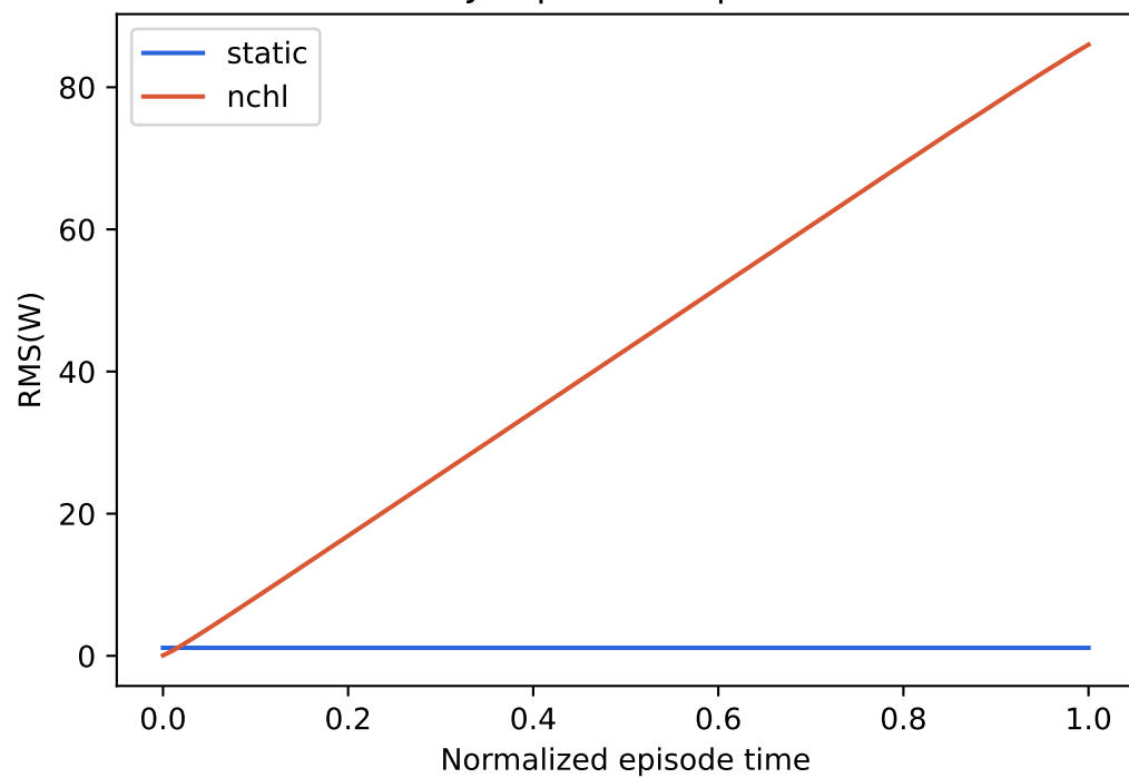
Thrower-v0 / thrower_arm
