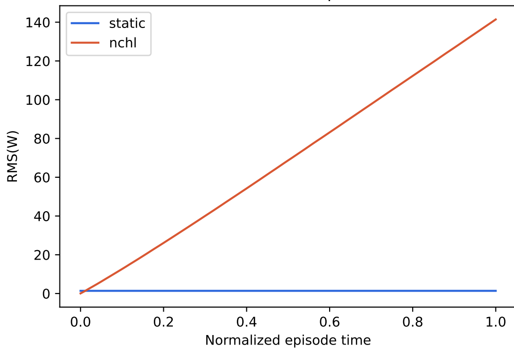
Walker-v0 / biped
