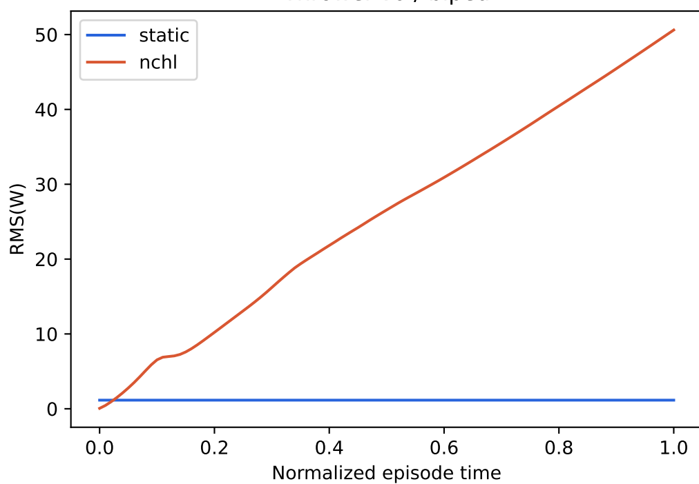
Walker-v0 / biped
