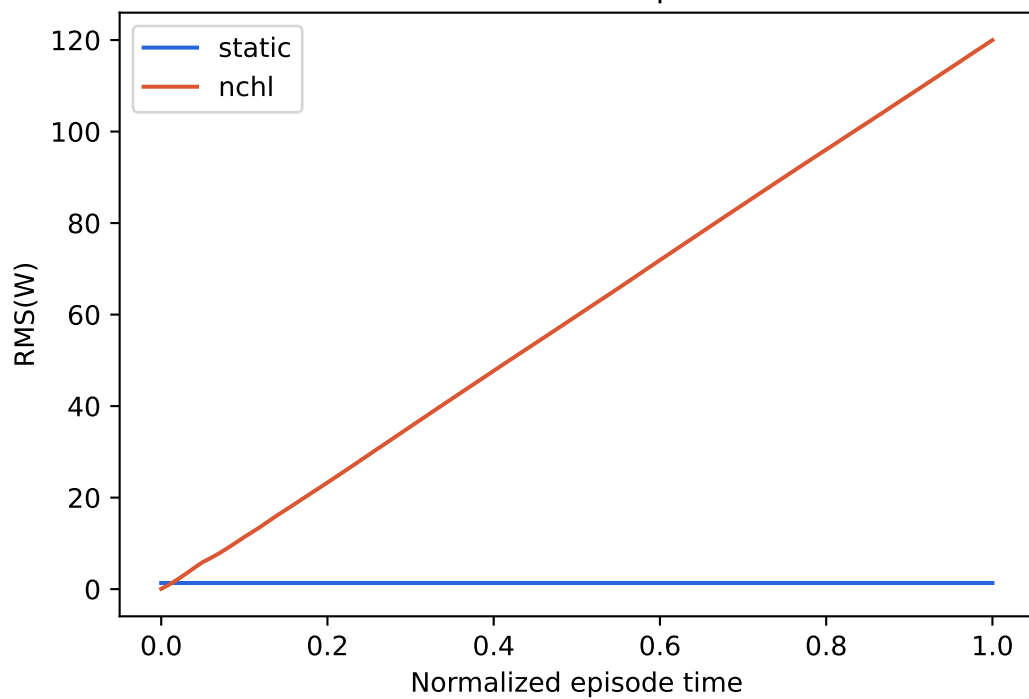
Thrower-v0 / biped
