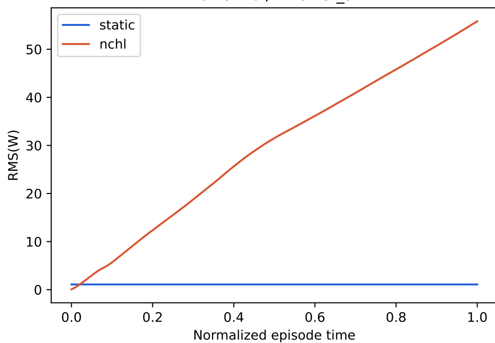
Thrower-v0 / thrower_arm
