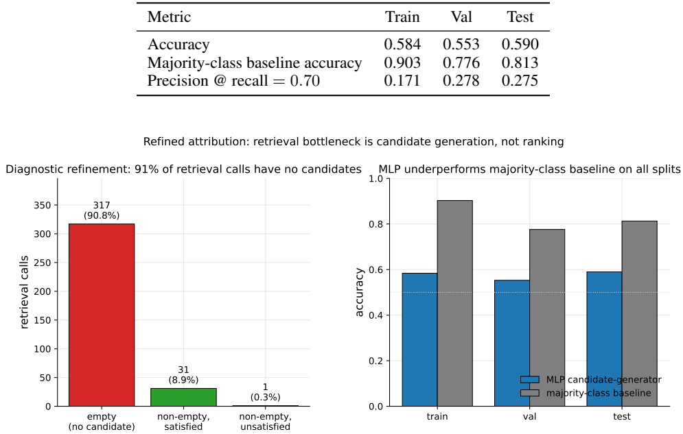
Figure 9: Refined attribution diagnostic. Left : 349 retrieval calls aggregated across 10 seeds; 317 (90.8%) returned empty candidate sets, 31 (8.9%) returned at least one satisfied candidate, only 1 (0.3%) returned candidates that were ranked but unsatisfied. The bottleneck is candidate generation, not candidate ranking. Right : the trained MLP underperforms a majority-class baseline on all three seed-disjoint splits, confirming that instantaneous state features alone are insufficient to predict candidate eligibility.
