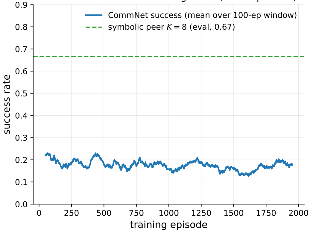
CommNet REINFORCE training curve (2000 episodes)
