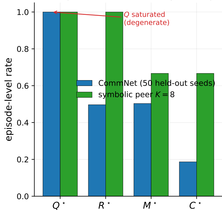
Q/R/M/C profile: CommNet vs symbolic peer
