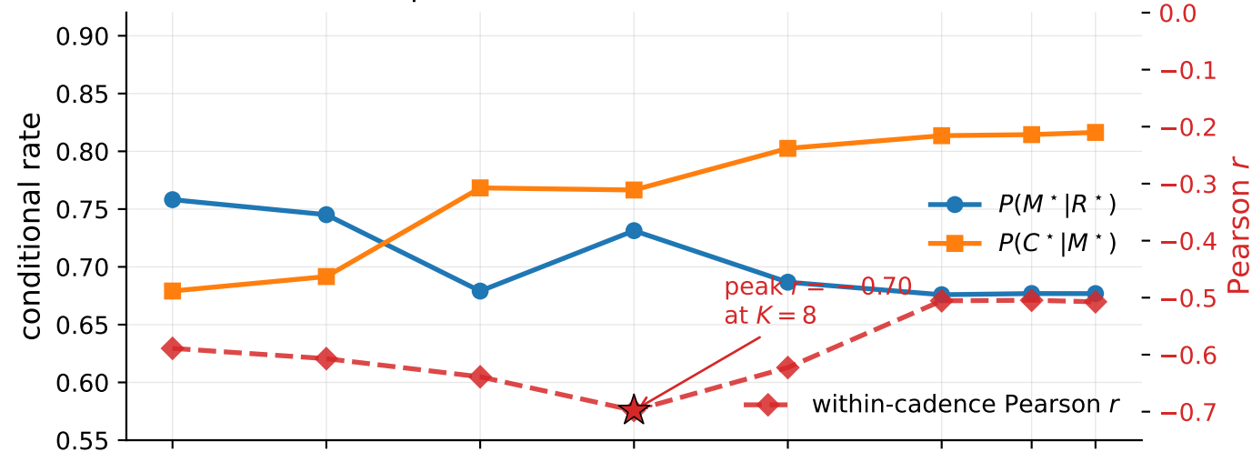
Interior minimum preserved at K = 8 ( t_{\text{succ}} = 4.77 )
