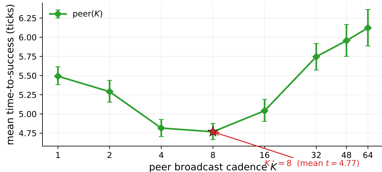
Interior minimum preserved at K = 8 ( t_{\text{succ}} = 4.77 )
