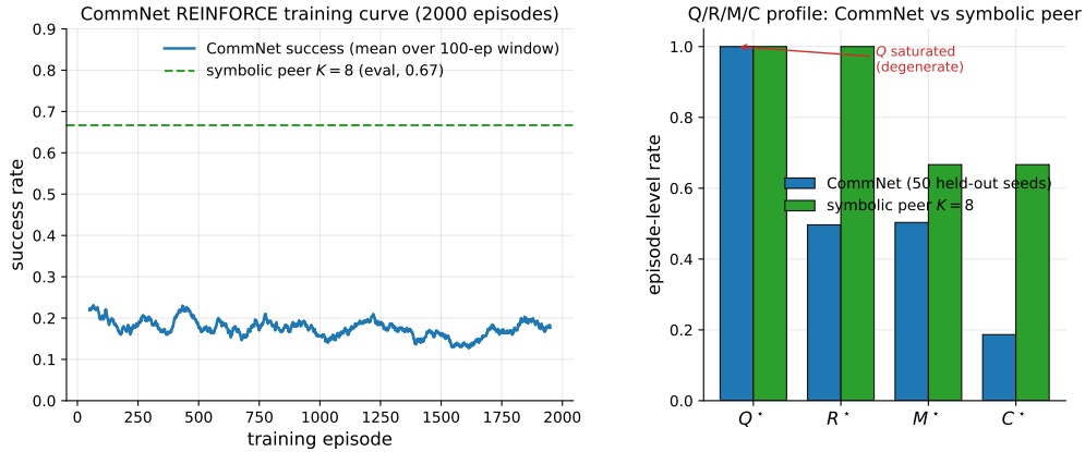
Figure 10: Learned-communication baseline diagnostics. Left : CommNet training curve (smoothed success rate over a 100-episode window) over 2000 training episodes; success stays below 0.25 throughout. The dashed line is the symbolic peer architecture at K=8 on the same scenario for reference. Right : Q/R/M/C profile of the trained CommNet on 50 held-out seeds vs symbolic peer at K=8 . Q^* is saturated at 1.0 on CommNet (degenerate by construction); R/M collapse together; only on the symbolic architecture are the conditional rates separated.
