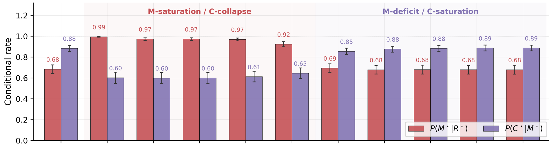
Per-architecture stage decomposition (35,640-run sweep, N \in \{3, 5, 8\} , 40 seeds)
