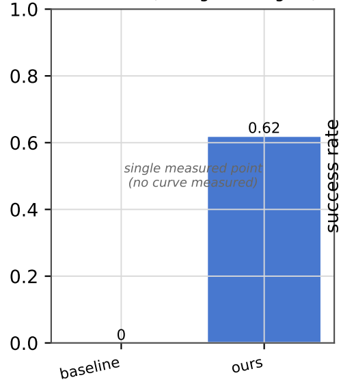
ALFWorld (task/grounding ↑)
