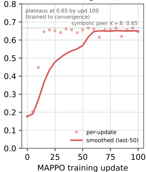
MARL baseline convergence (measured)
