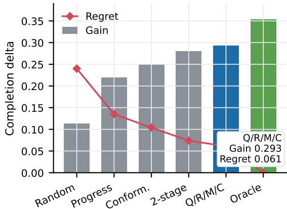
(b) Repair selected by diagnosis
