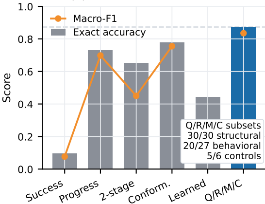
(a) Blinded fault localization
