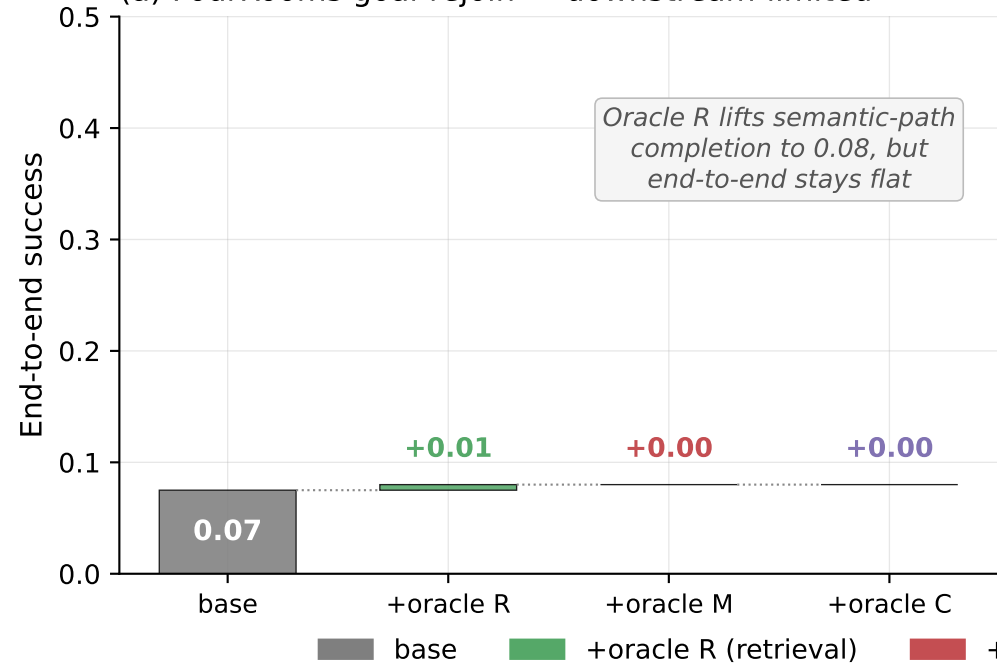
(a) FourRooms goal-rejoin — downstream-limited
