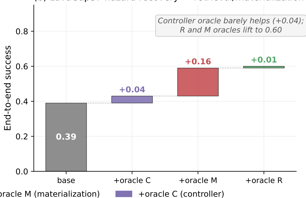
(b) LavaGapS7 hazard recovery — retrieval/materialization-limited
