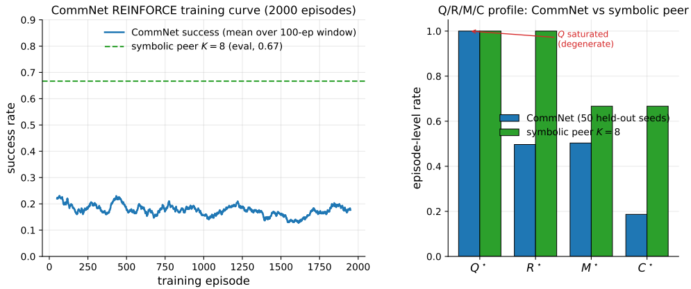
Figure 12: Learned-communication baseline diagnostics. Left: CommNet training curve (smoothed success rate over a 100-episode window) over 2000 training episodes; success stays below 0.25 throughout. The dashed line is the symbolic peer architecture at K=8 on the same scenario for reference. Right: Q/R/M/C profile of the trained CommNet on 50 held-out seeds vs symbolic peer at K=8 . Q^* is saturated at 1.0 on CommNet (degenerate by construction); R/M collapse together; only on the symbolic architecture are the conditional rates separated.
