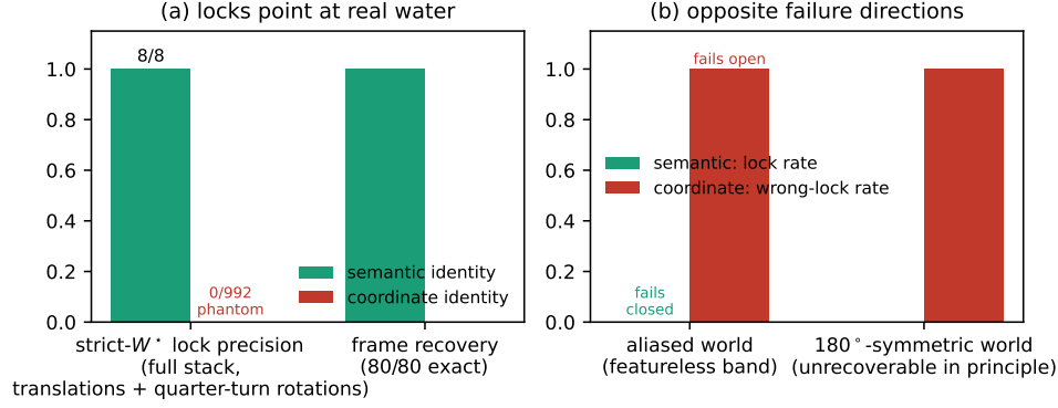
Figure 19: Meaning-based identity under SE(2) frames. (a) Every strict- W^* lock the semantic stack makes points at real water (8/8); the coordinate stack makes 992 locks, all phantoms (0/992); frame recovery itself is exact in 80/80 witness-traveler combinations. (b) The failure asymmetry in worlds where identification is impossible (featureless band; a 180°-symmetric layout where the frame is unrecoverable in principle): semantic identity refuses to lock — fails closed — while coordinate identity keeps confidently locking wrong cells — fails open.
