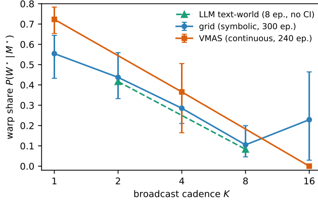
Figure 16: One quantity, three substrates: warp share P(W^*|M^*) vs. broadcast cadence K on the symbolic grid, the continuous VMAS scenario, and the LLM text-world. The curves nearly coincide — how much of a collective’s materialisation runs on foreign evidence is set by the sharing cadence, not by the substrate. (LLM arm: 8 episodes, point estimates only.)
