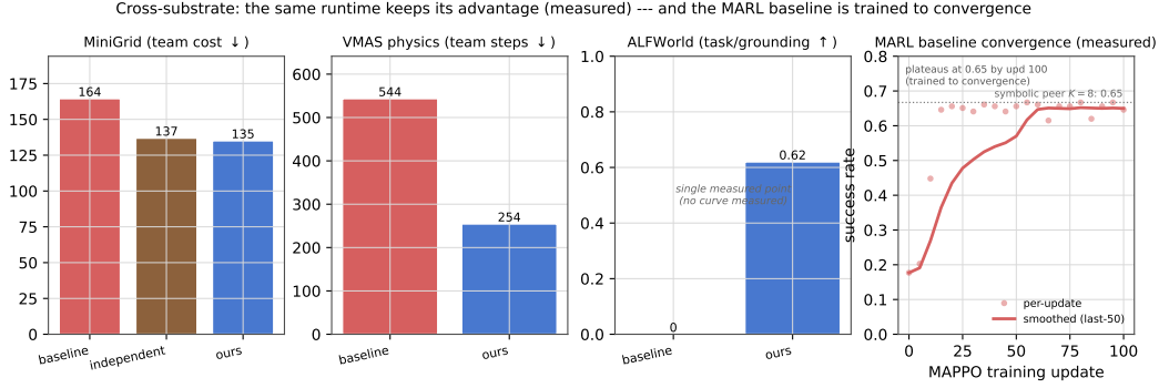
Figure 26: The integrated runtime keeps its advantage across substrates (measured summaries): MiniGrid team cost and VMAS physics team steps (lower is better), and ALFWorld task grounding (single measured point; no convergence curve was measured). The fourth panel is the measured MAPPO baseline training curve, which plateaus at success \approx 0.65 — the symbolic-peer K=8 level — confirming the multi-agent-RL baseline is trained to convergence, so the runtime’s advantage is not an artefact of an undertrained baseline.
