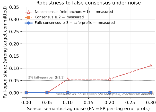
Figure 25: Fail-closed safety under sensor noise (measured N1 sweep, 24 seeds/cell, diagonal FN=FP). Removing the anchor-consensus mechanism (min-anchors = 1) lets the fail-open rate climb above the 5% bar as tag noise grows; anchor consensus \geq 2 and the full consensus \geq 3 + safe-prefix arm hold fail-open at 0.000 across the whole sweep — degrading into refusals (a coverage cost) rather than wrong commitments.
