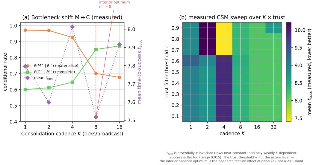
Figure 22: (a) The materialization–completion bottleneck shift and the interior time-to-success optimum at K^*=8 , measured on the same 35,640-run peer-broadcast sweep (Fig. 21): P(M^*|R^*) falls and P(C^*|M^*) rises with K , while mean t_{succ} has an interior minimum. (b) The measured CSM sweep over cadence K and trust threshold \tau : mean t_{succ} is essentially \tau -invariant and only weakly K -dependent, and mission success is flat in (K, \tau) (range 0.015). The trust threshold is not the active lever in this regime — the interior operating point is the cadence effect of panel (a), not a two-dimensional optimum island.
