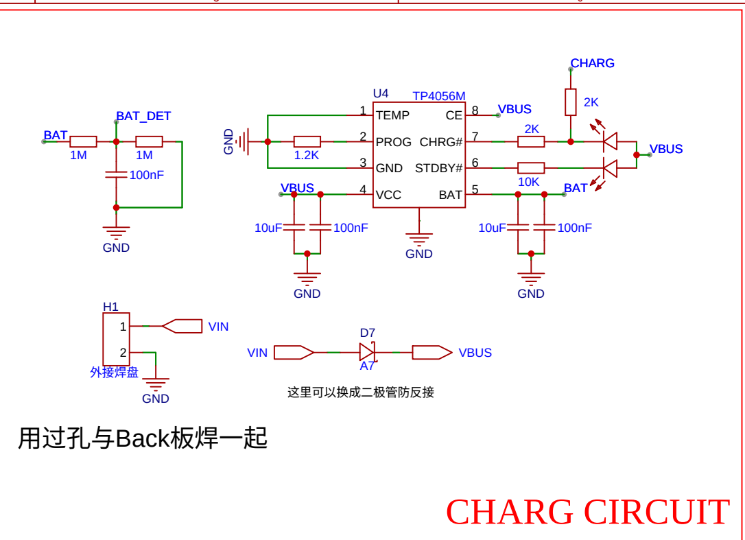
POWER SUPPLY
