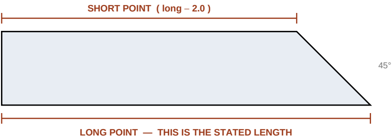
DETAIL A — WHICH LENGTH IS THE PART NUMBER? scale 1:2.6
