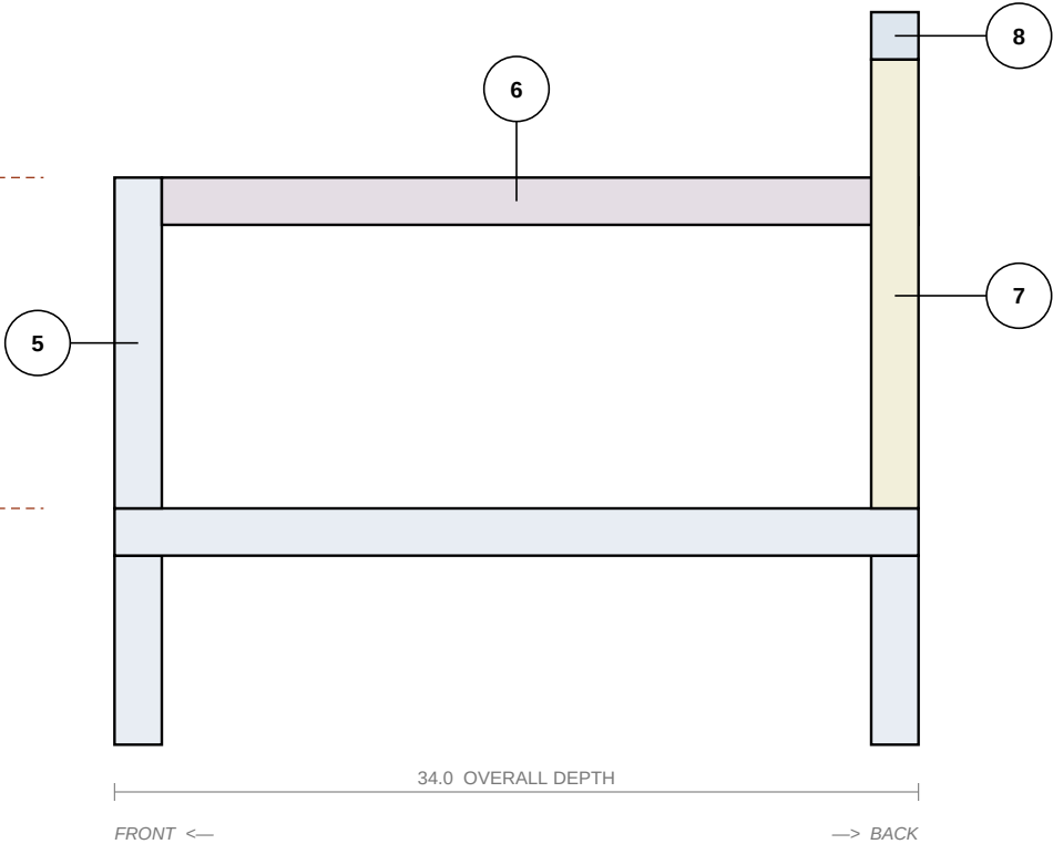
SIDE ELEVATION scale 1:9 · left side shown, right side identical
