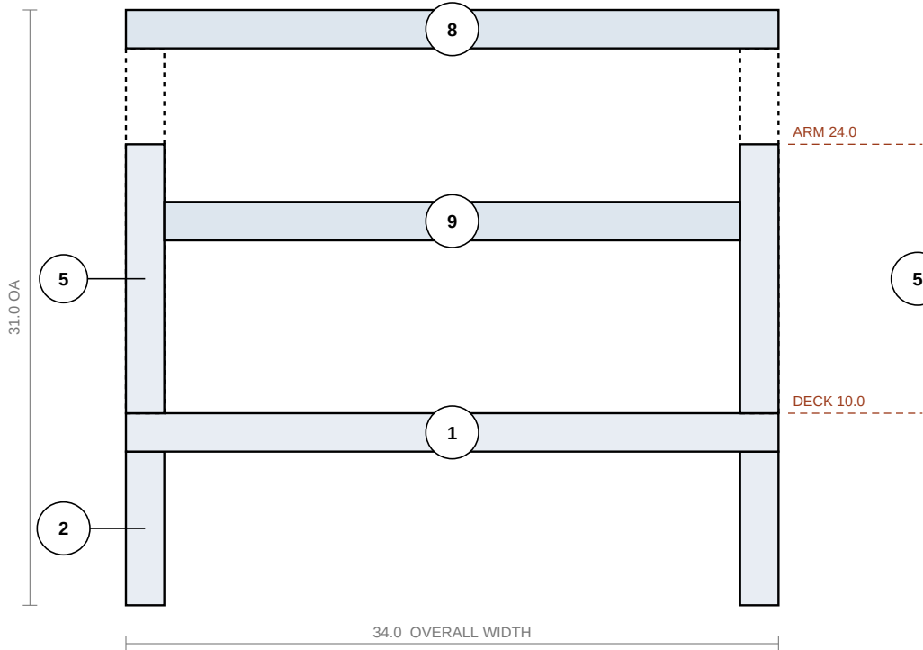
FRONT ELEVATION scale 1:9
