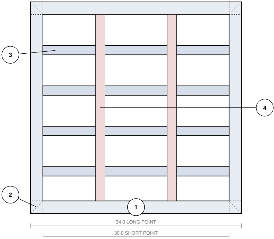
PLAN — SEAT FRAME ASM-BRV-SEAT-034x034 · scale 1:9 · cushion + back removed
