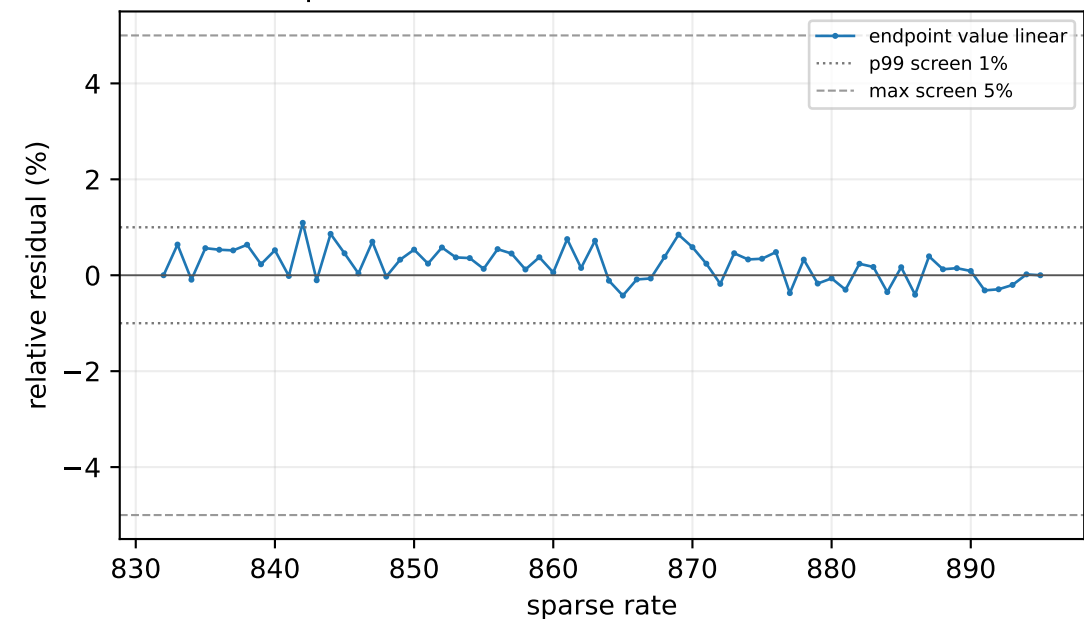
E2M1 pointwise relative residual (R896 excluded)
