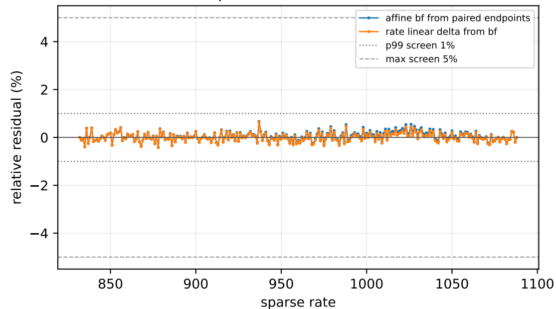
E4M3 pointwise relative residual
