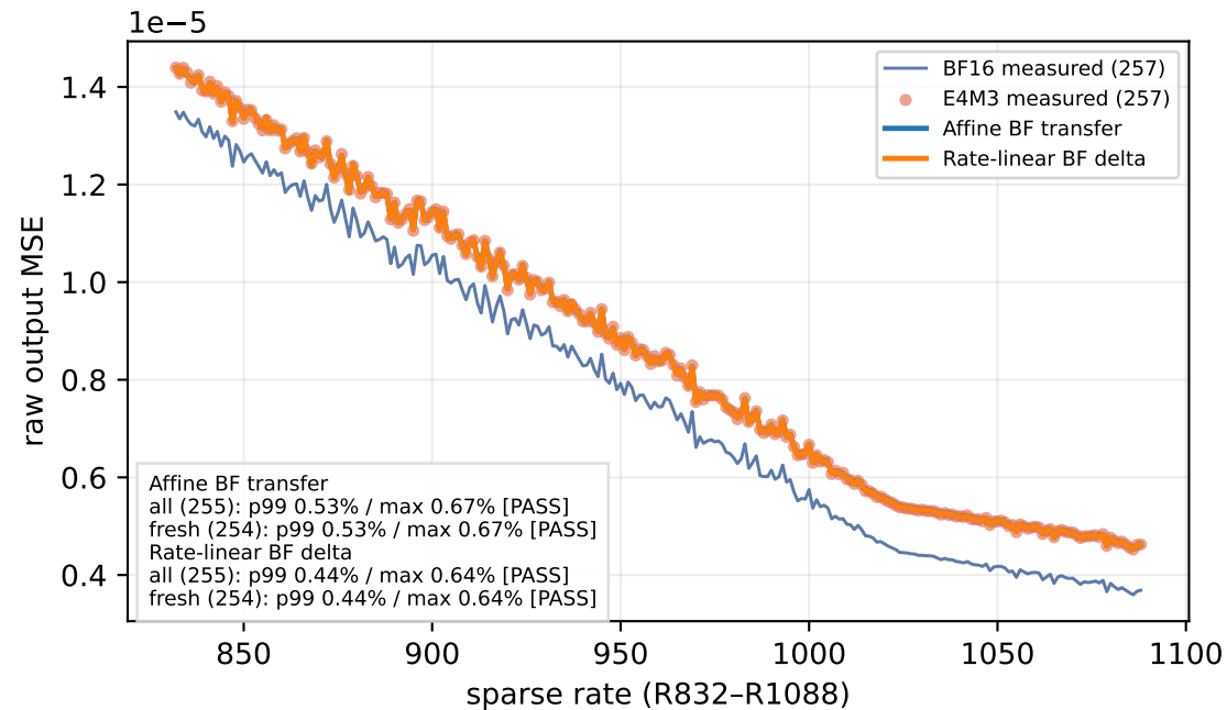
E4M3 transfer: measured curve and sealed predictions
