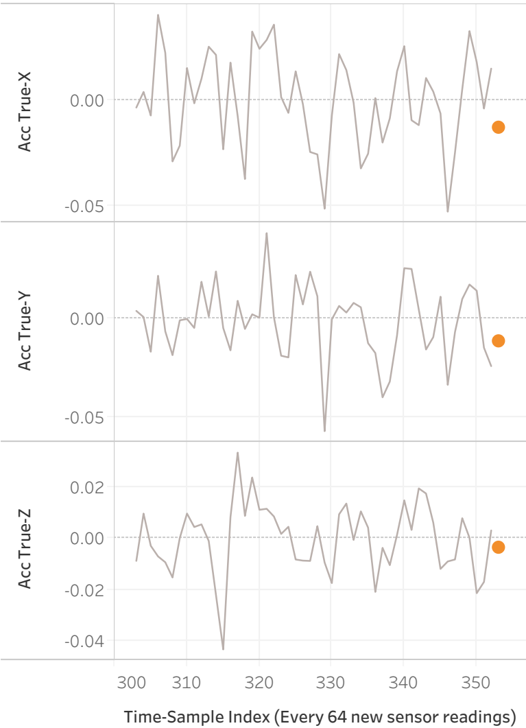
Recent Sensor Mean-Readings Next Time Step Forecast (Accelerometer)
