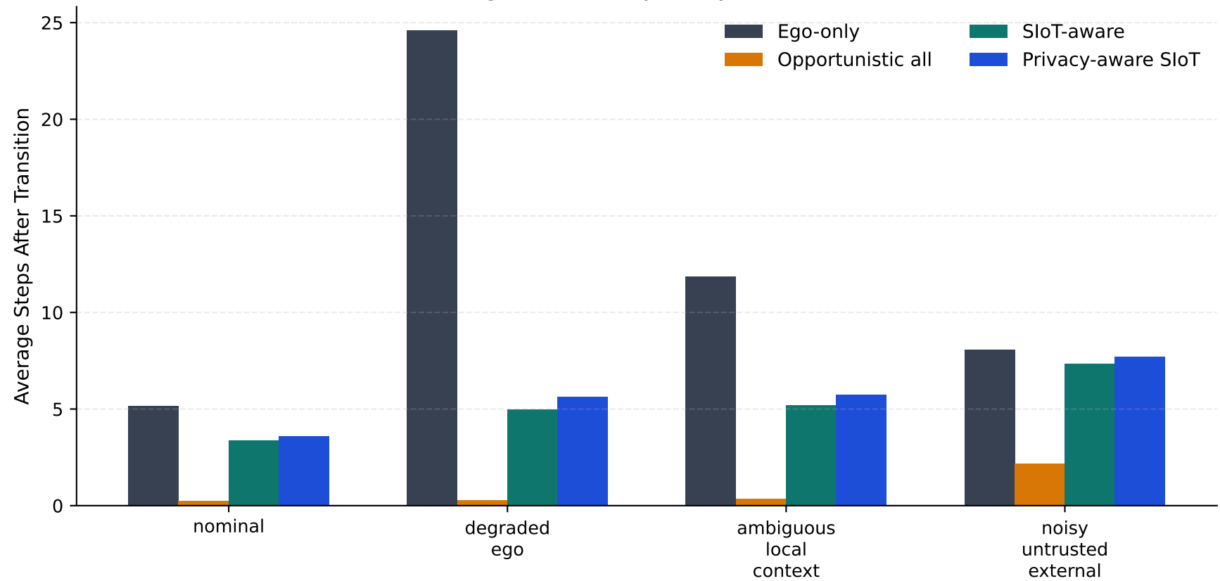
Convergence Time by Policy and Scenario
