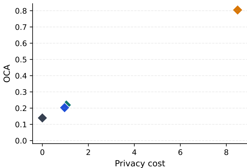
Ambiguous local
