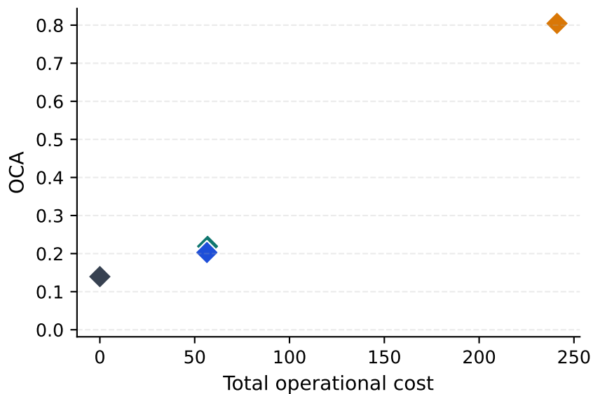
Ambiguous local
