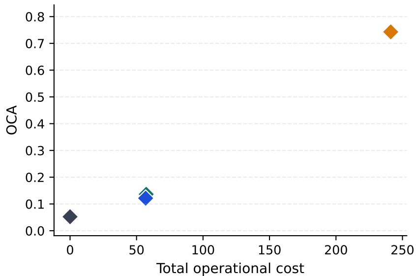
Ambiguous local
