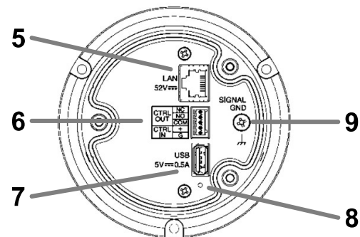
Rear Panel without Back Cover
