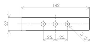
Bracket Dimensions
