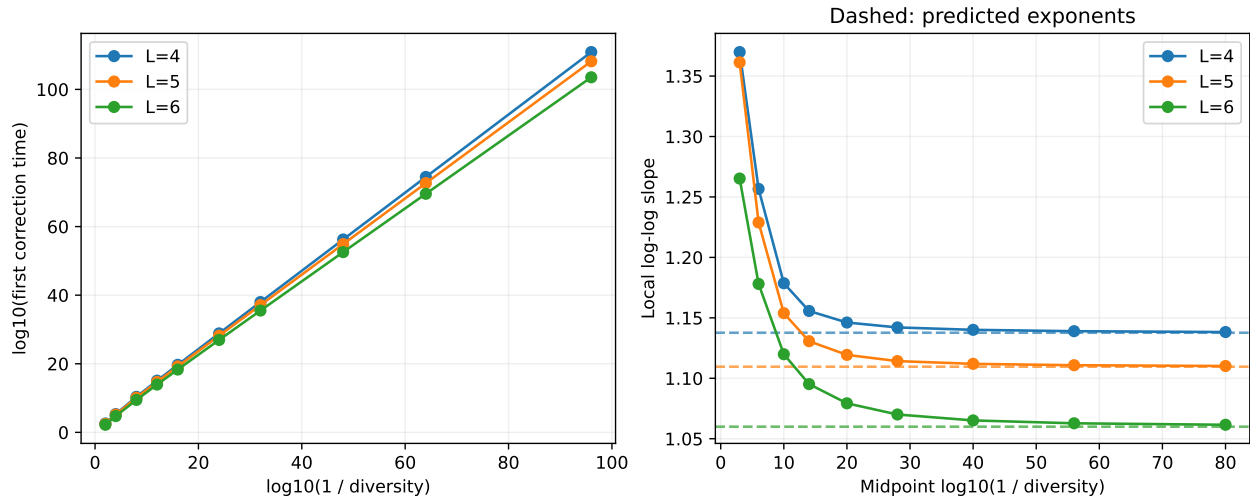
Figure 1: First correction times and successive log-log slopes from the retained numerical runs. Dashed lines show the theorem’s exponents. The finite-range slopes are evidence about convergence, not a proof of it.
