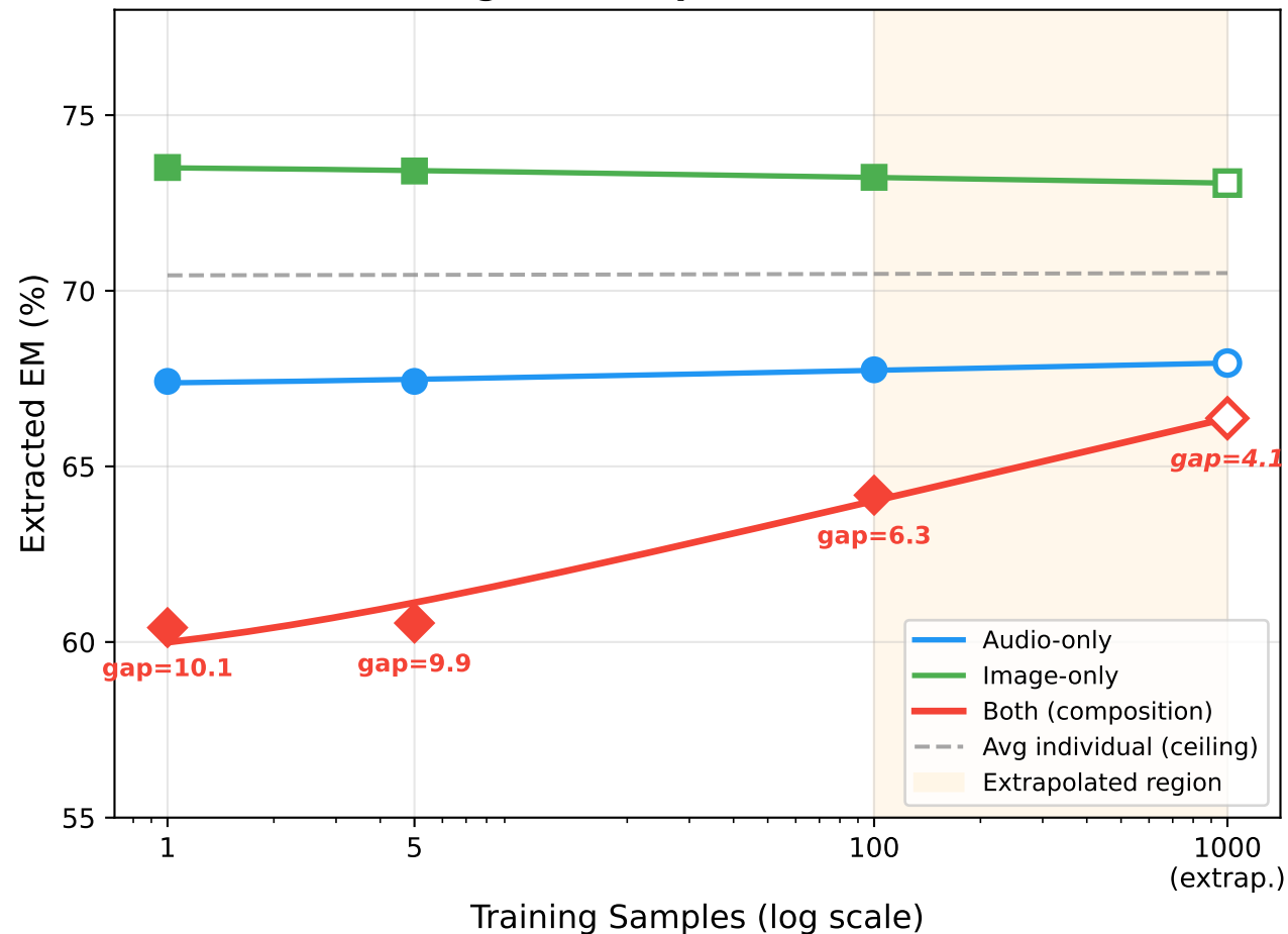
Calibration Sweep: Accuracy vs Data Volume (with log-fit extrapolation to n=1000)
