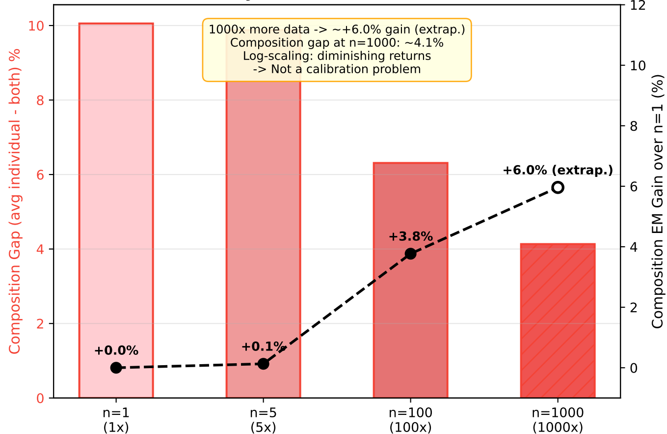
Composition Gap Persists Despite Polynomial Data Increase
