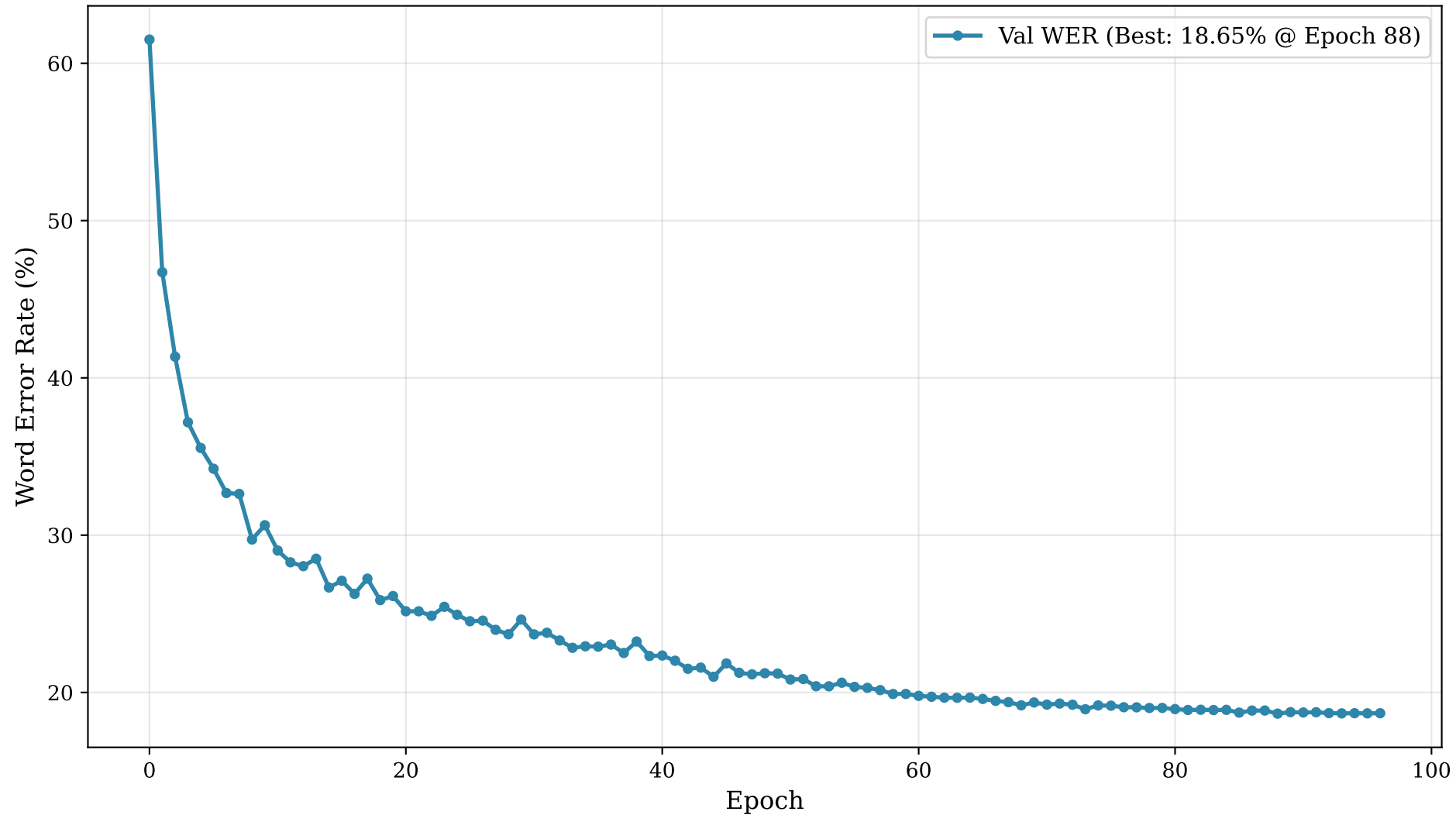
Validation WER During Training
