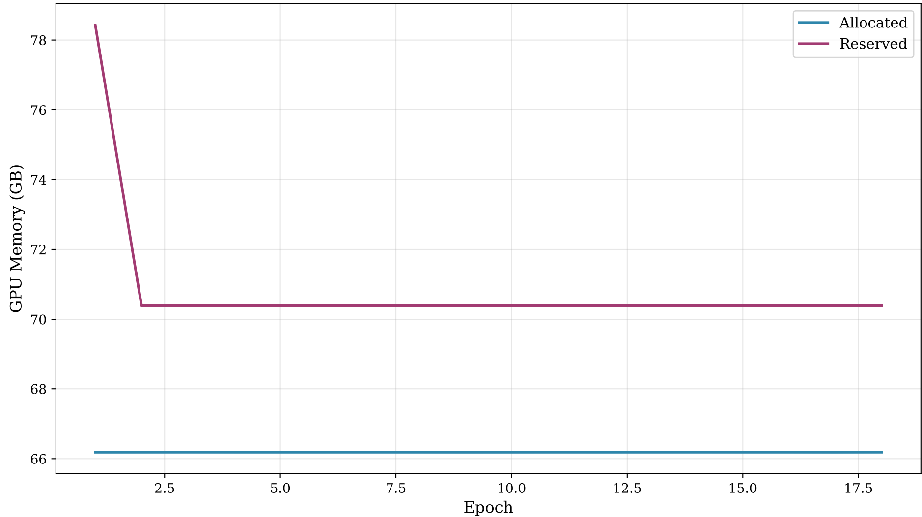
GPU Memory Usage During Training
