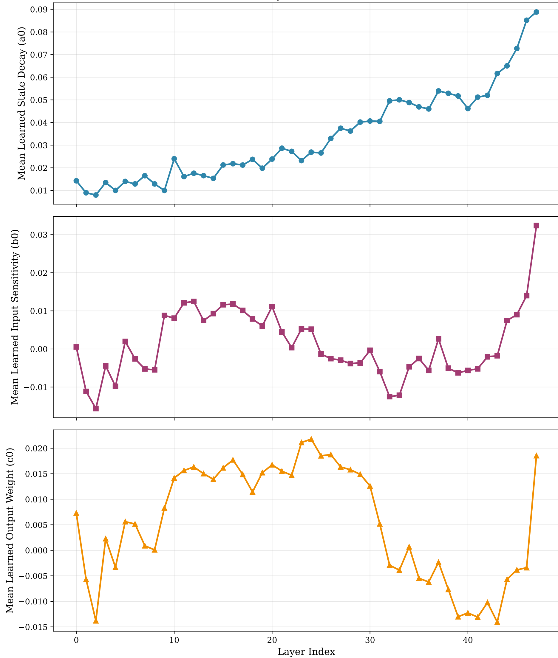
Learned Hierarchical Dynamics (Mean Parameter Values)
