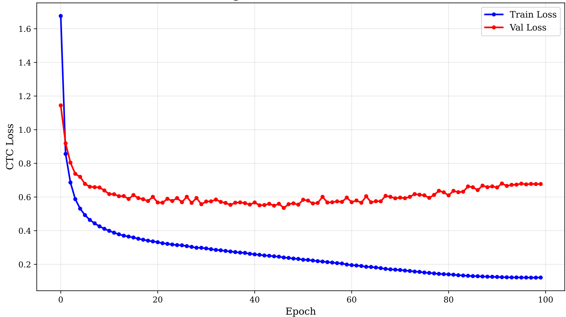
Training and Validation Loss Curves
