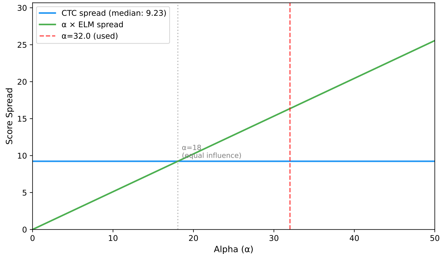
CTC vs ELM Score Influence as \alpha Increases
