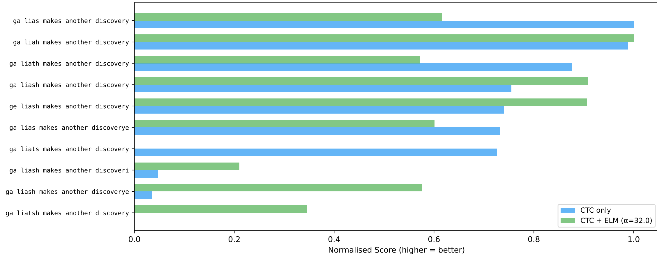
Rescoring Effect — Ref: "goliath makes another discovery"
