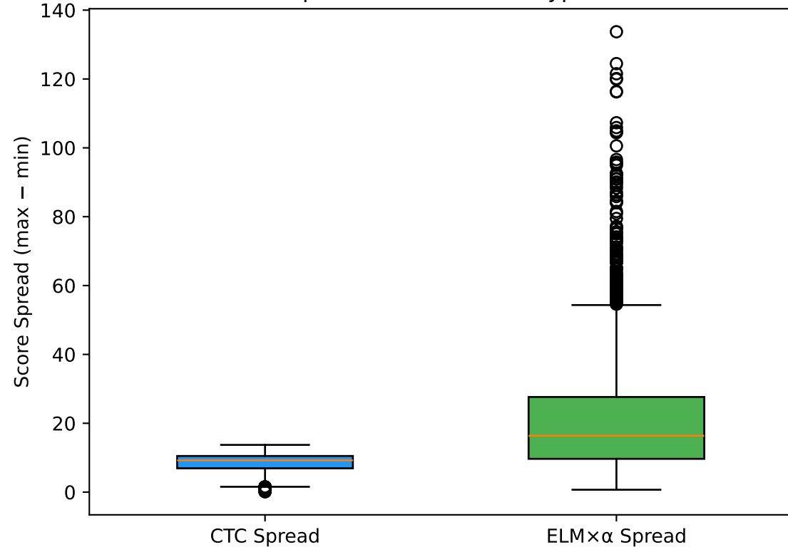
Score Spread Across Beam Hypotheses
