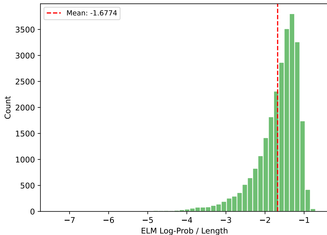
Score Spread Across Beam Hypotheses
