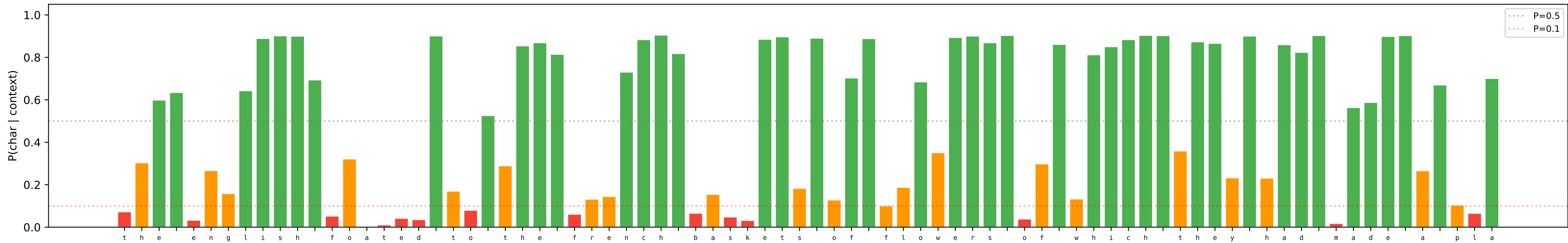
Per-Character ELM Probability: "the english foated to the french baskets of flower..." [confirmed]
