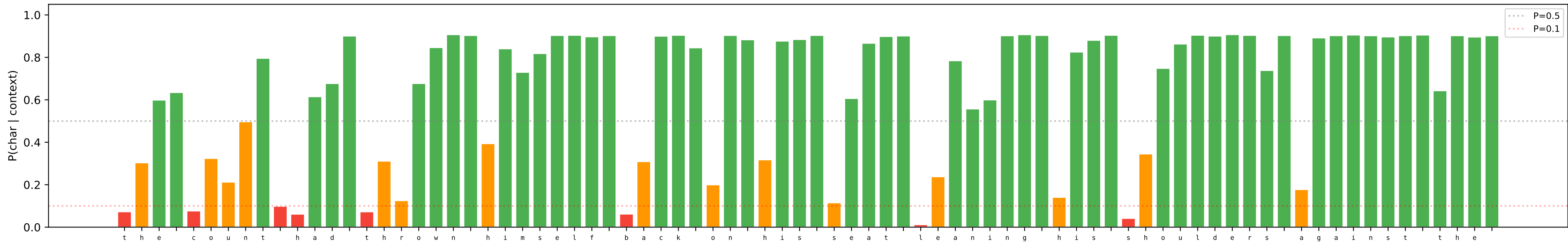
Per-Character ELM Probability: "the count had thrown himself back on his seat lean..." [RE-RANKED]
