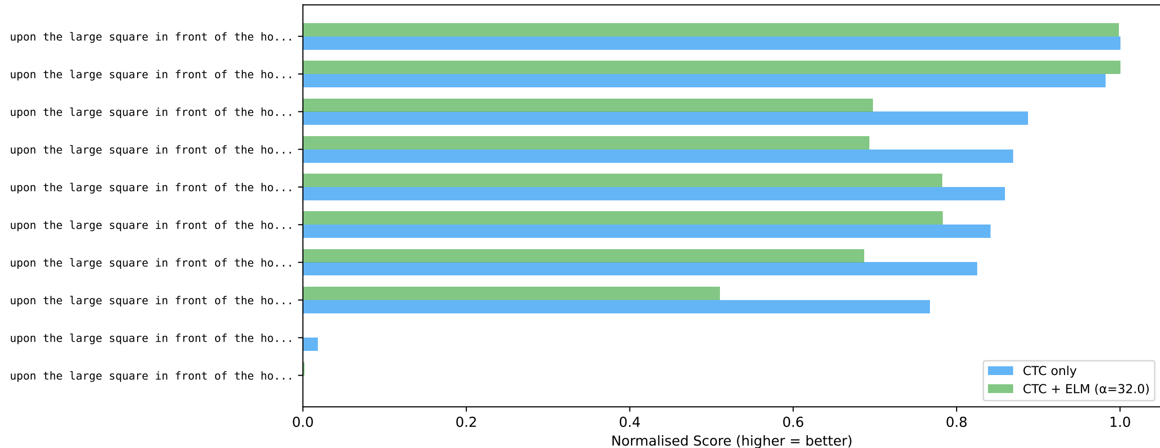
Rescoring Effect — Ref: "upon the large square in front of the hotel the shadows of the tents i..."
