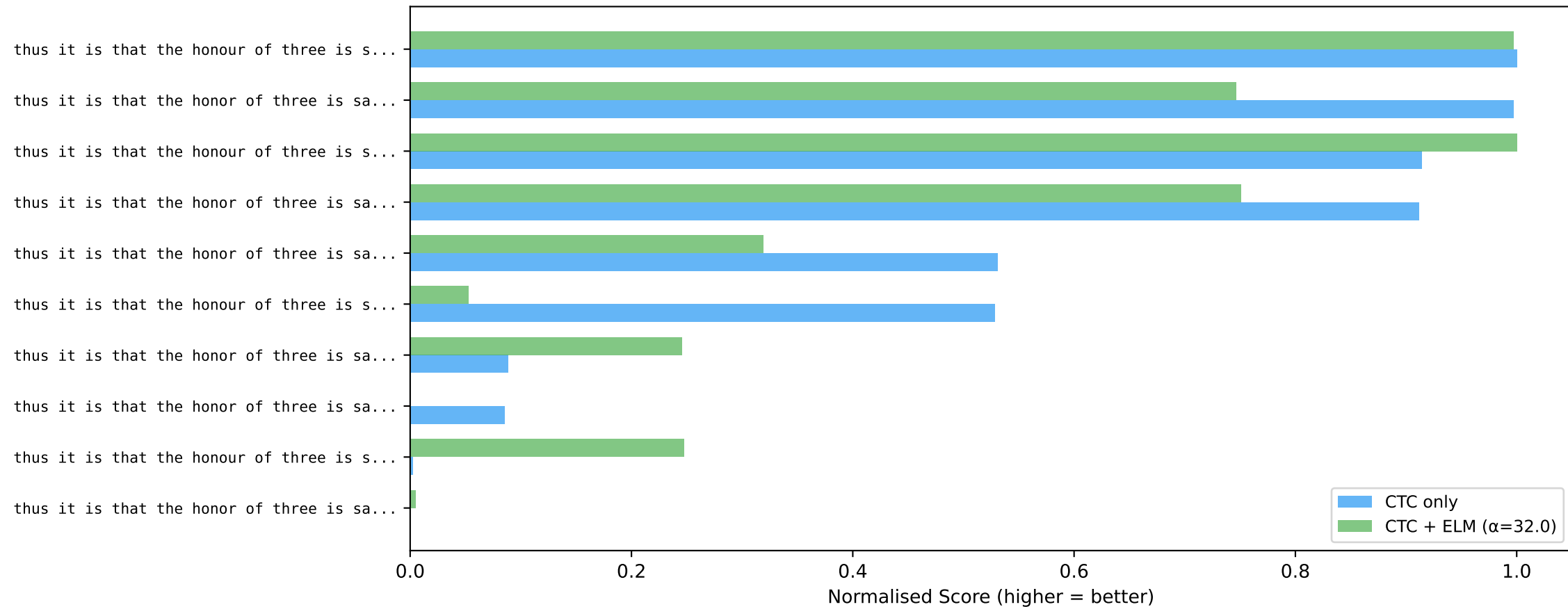
Rescoring Effect — Ref: "thus it is that the honor of three is saved our country's our master's..."
