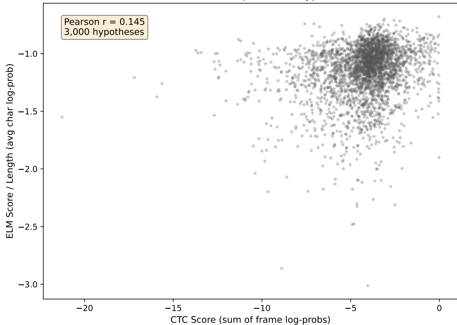
CTC vs ELM Score per Beam Hypothesis
