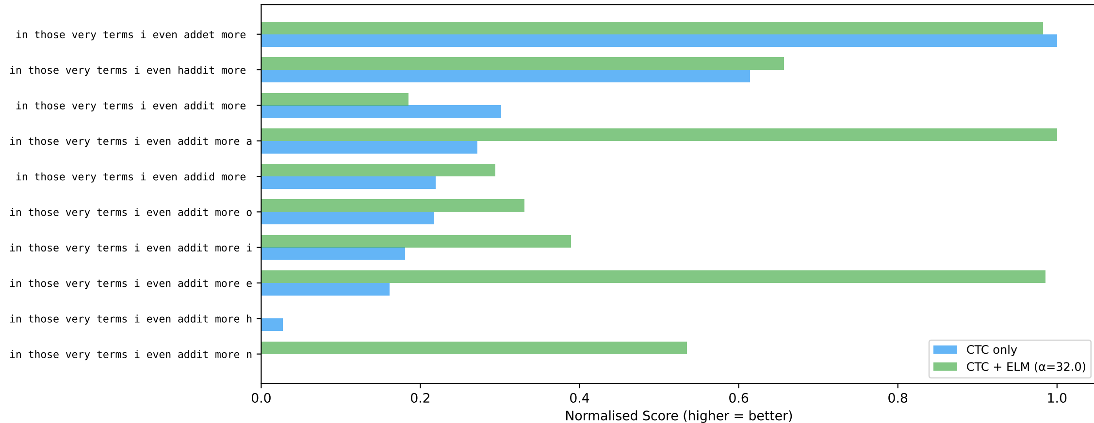
Rescoring Effect — Ref: "in those very terms i even added more"
