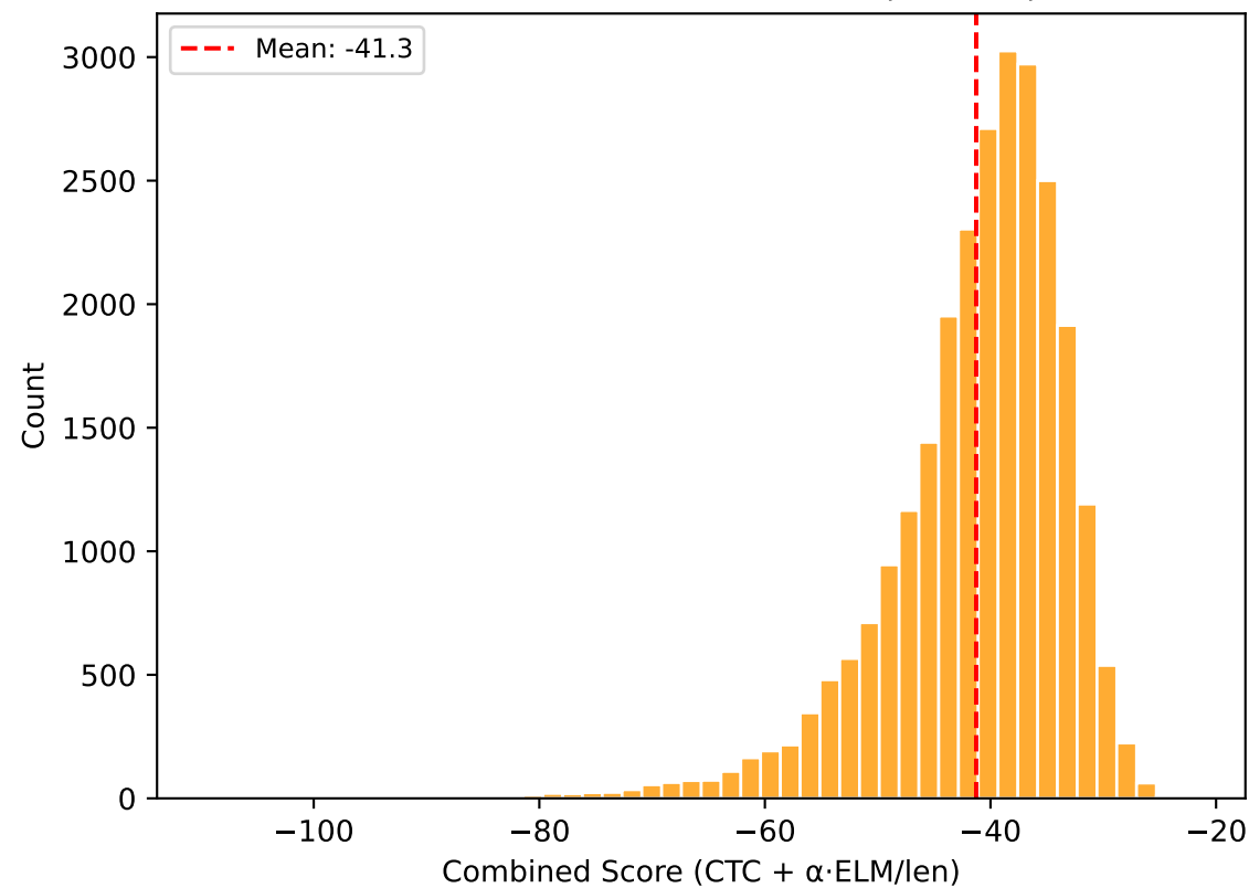
Combined Score Distribution ( \alpha=32.0 )
