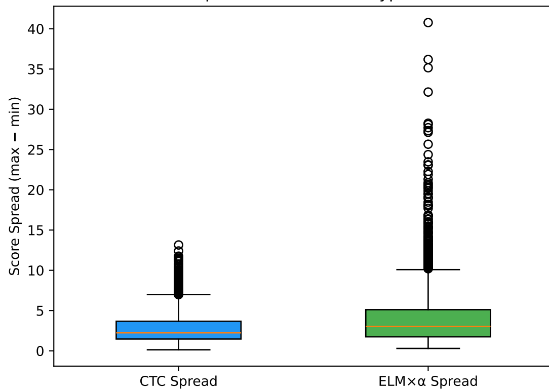
Score Spread Across Beam Hypotheses
