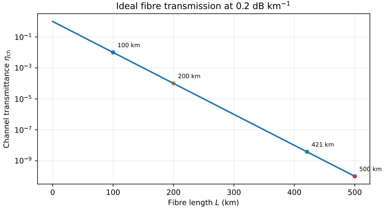
FIG. 3. Calculated transmission through optical fibre with attenuation \alpha = 0.2 \text{ dB/km} , using equation (16) . The vertical axis is logarithmic. Transmission falls exponentially with fibre length, limiting the detected signal in a direct link. This loss motivates lower-loss fibre, improved detectors, alternative link geometries and quantum repeaters.
