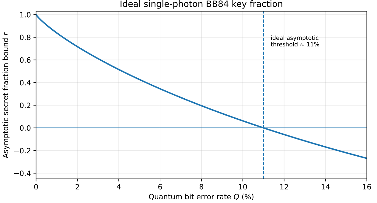
FIG. 2. Asymptotic single-photon BB84 secret-fraction bound from equation (12) . The bound falls to zero at a QBER of approximately 11% under the assumptions stated in the text. The figure is a theoretical benchmark, not a universal operating threshold for all QKD protocols.
