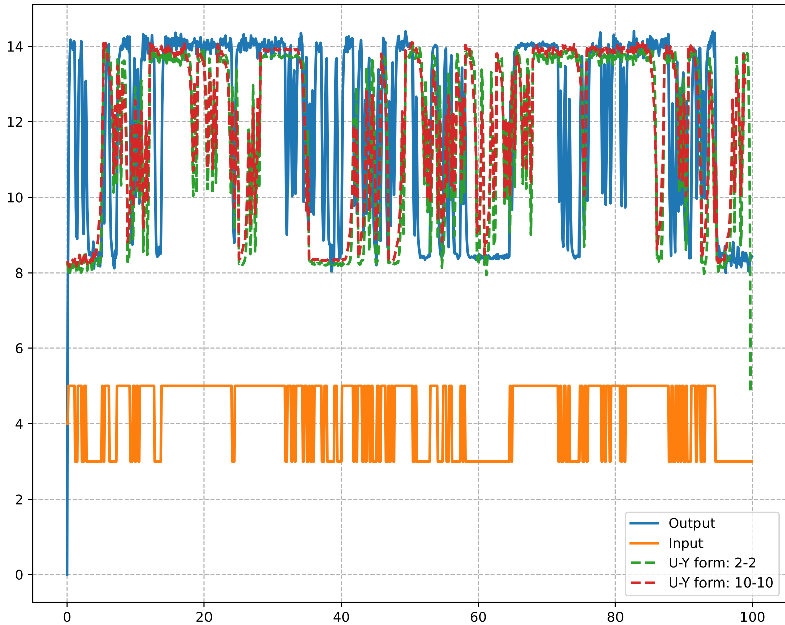
Input/Output vs IDed Output for Best Model: System 1,2,3 Combined
