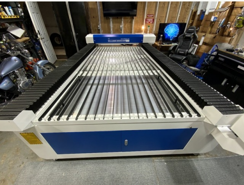
CO2 laser | Cutting and engraving bed
