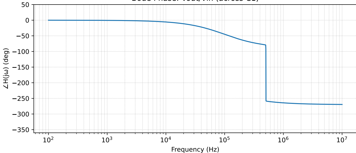
Bode Phase: V_{out}/V_{in} (across C1)
