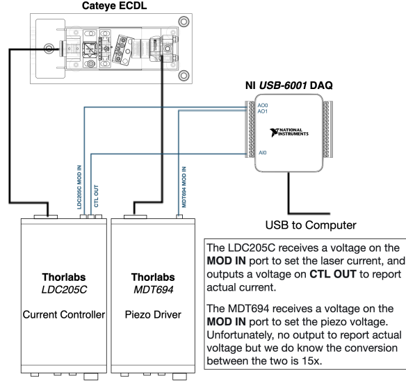
Figure 6: Schematics for the digital feedforward circuit
