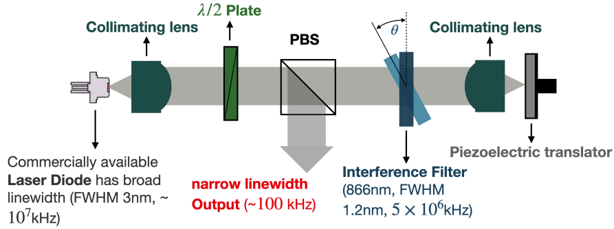
Figure 3: Schematics of Cateye IF ECDL Optics
