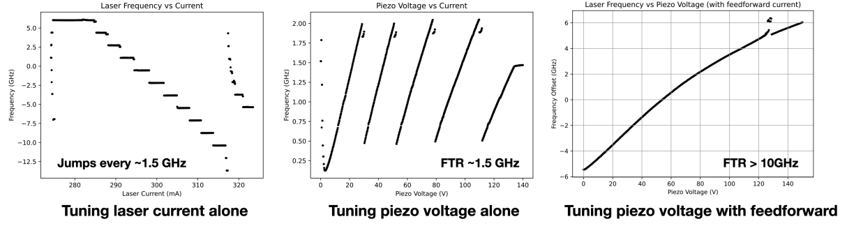
Figure 7: Laser output frequency as scanning laser current alone (left), scanning piezo voltage alone (middle), and scanning piezo voltage with feedforward (right)
