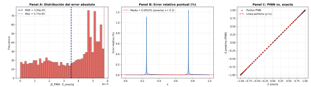
Fig. 2. Additional training metrics for NB01. Panel A: distribution of the absolute error |\hat{E}(x) - E_{\text{exact}}(x)| . Panel B: pointwise relative error (%). Panel C: scatter of the PINN prediction against the exact solution, with the y = x line as a perfect-fit reference.
