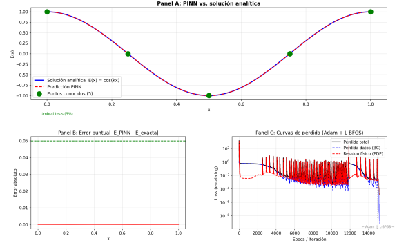
Fig. 1. PINN-SIREN validation for 1D Helmholtz. (a) Comparison between the network prediction and the analytical solution E_{\text{exact}}(x) = \cos(kx) at 1,000 uniform points in [0, 1] . (b) Pointwise error |\hat{E}(x) - E_{\text{exact}}(x)| . L^2 error = 0.006%, R^2 = 1.000000 . GPU: NVIDIA RTX 5050, SEED = 42.
