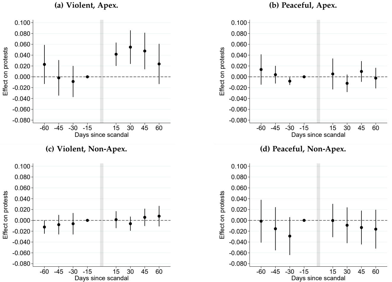
Figure 1. Protest dynamics: Apex vs. Non-Apex ( \pm 60 -day window, 15-day bins).
