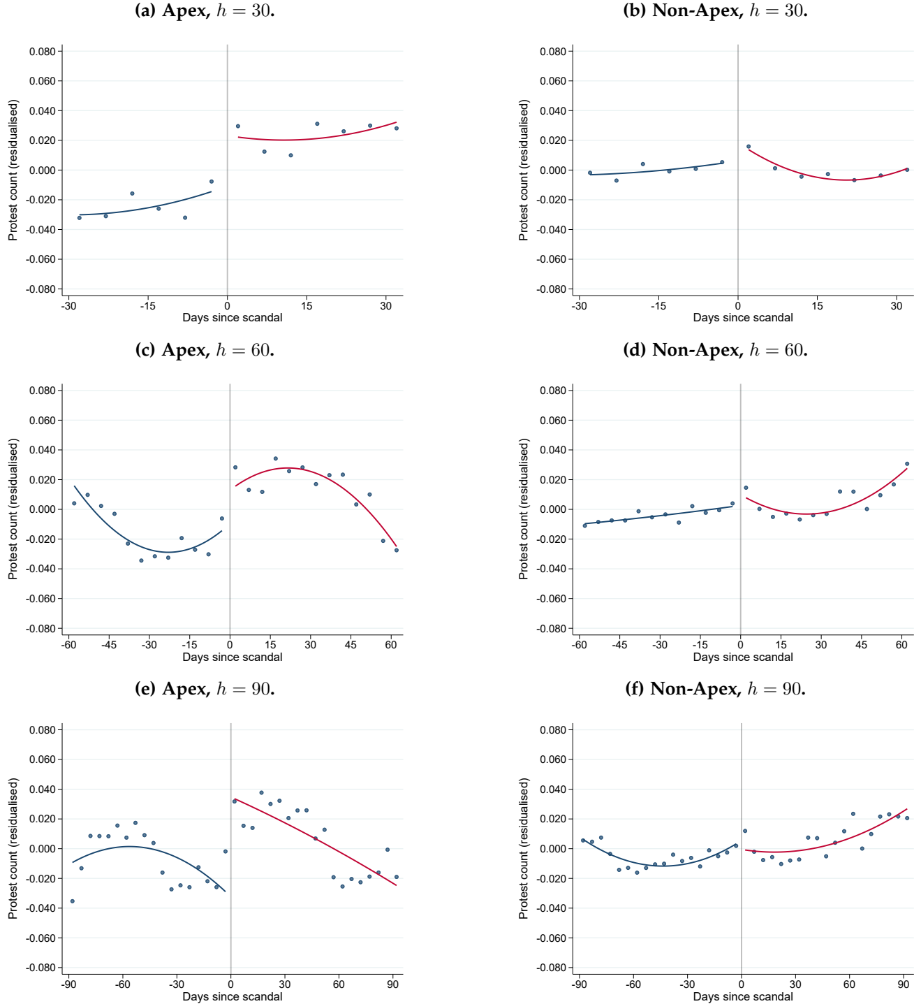
Figure S7. Regression discontinuity in event time, local-quadratic fit, violent protests, at h = 30/60/90 -day bandwidths.
