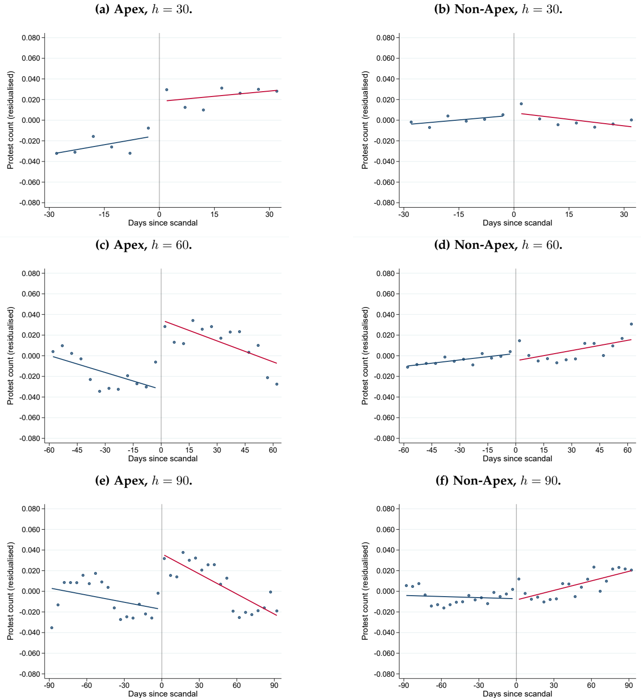
Figure S6. Regression discontinuity in event time, violent protests, at h = 30/60/90 -day bandwidths.
