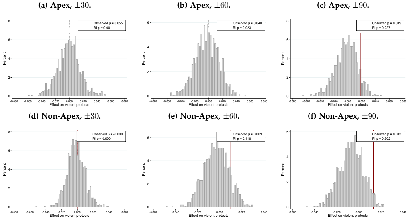
Figure S1. Randomization inference: violent protests.
