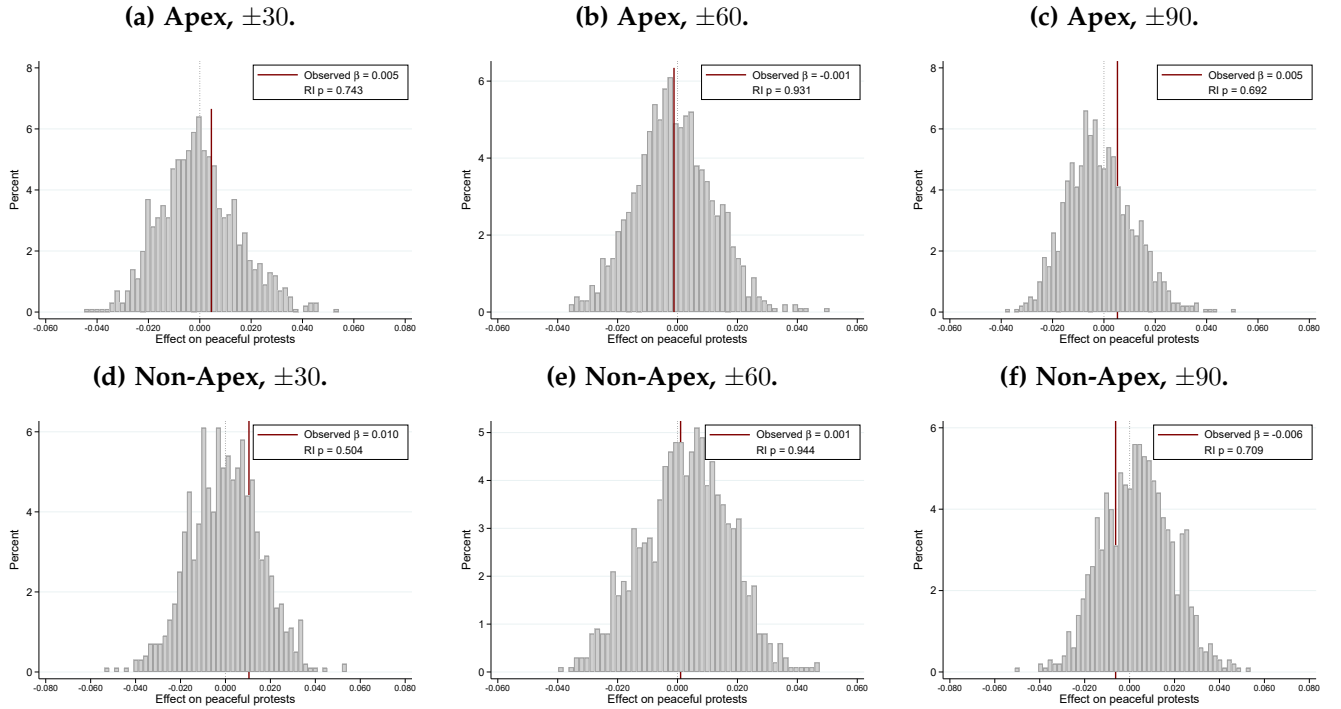
Figure S2. Randomization inference: peaceful protests.
