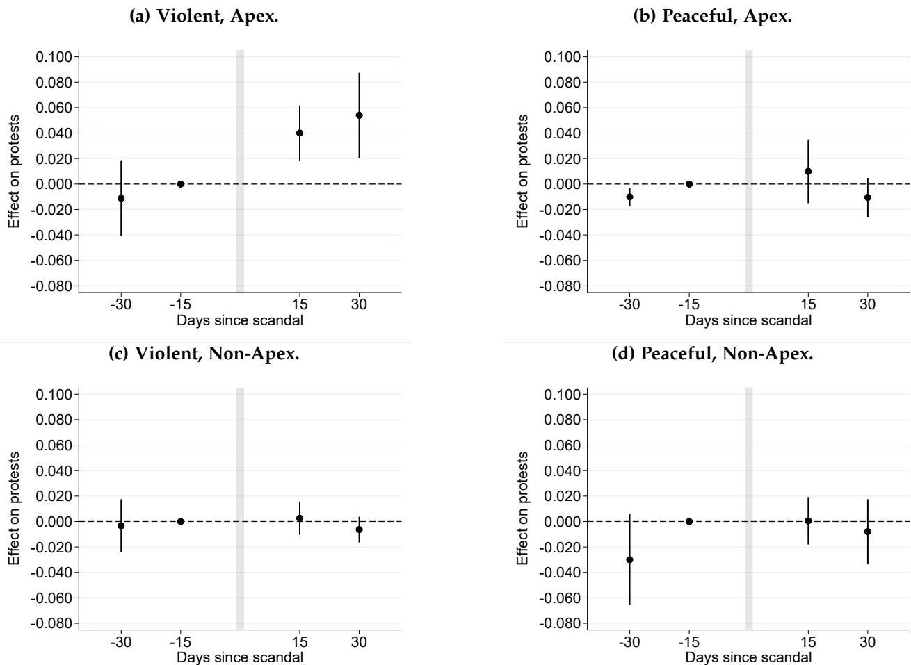
Figure S4. Event studies, \pm 30 -day window (15-day bins).
