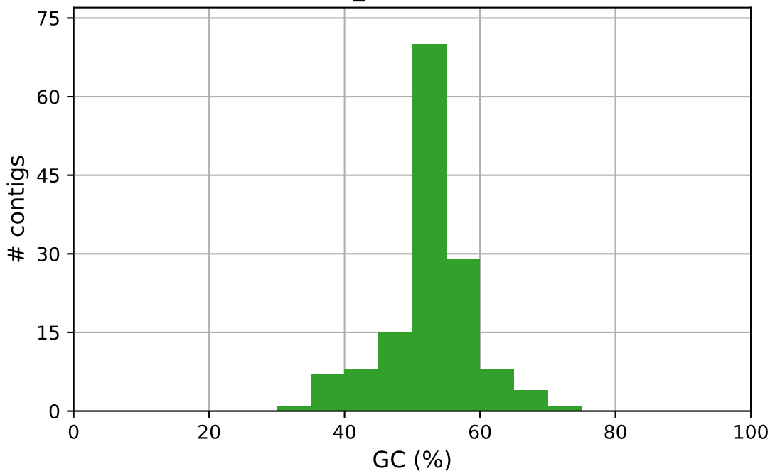
Velvet_k31 GC content
