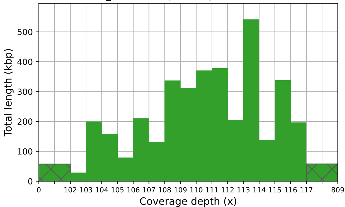
Velvet_k31 coverage histogram (bin size: 1x)
