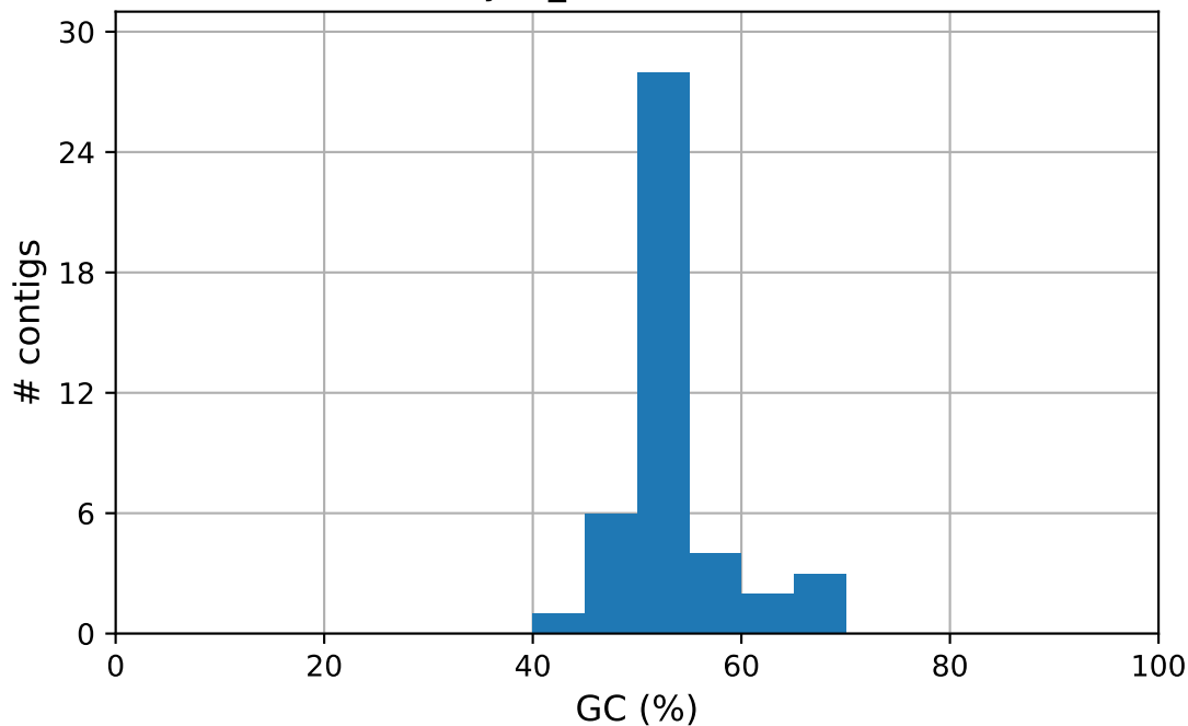
ABySS_k85 GC content
