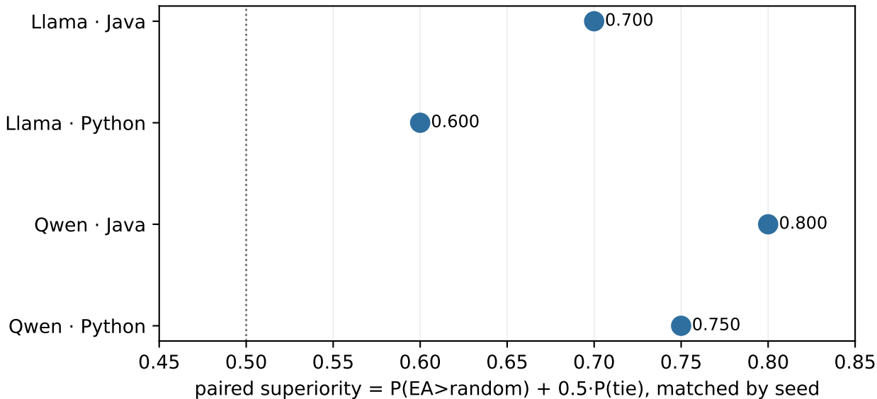
RQ2 — descriptive paired advantage after safe-zone filtering
