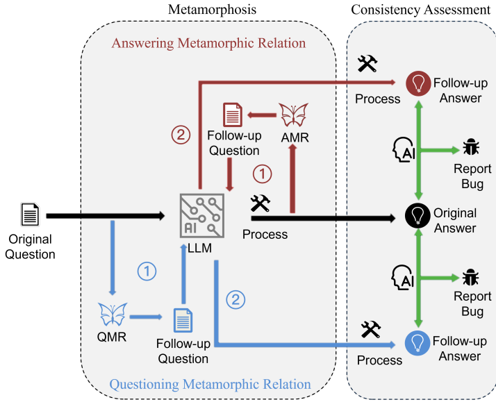
Fig. 2. A high-level overview of DrHall.
