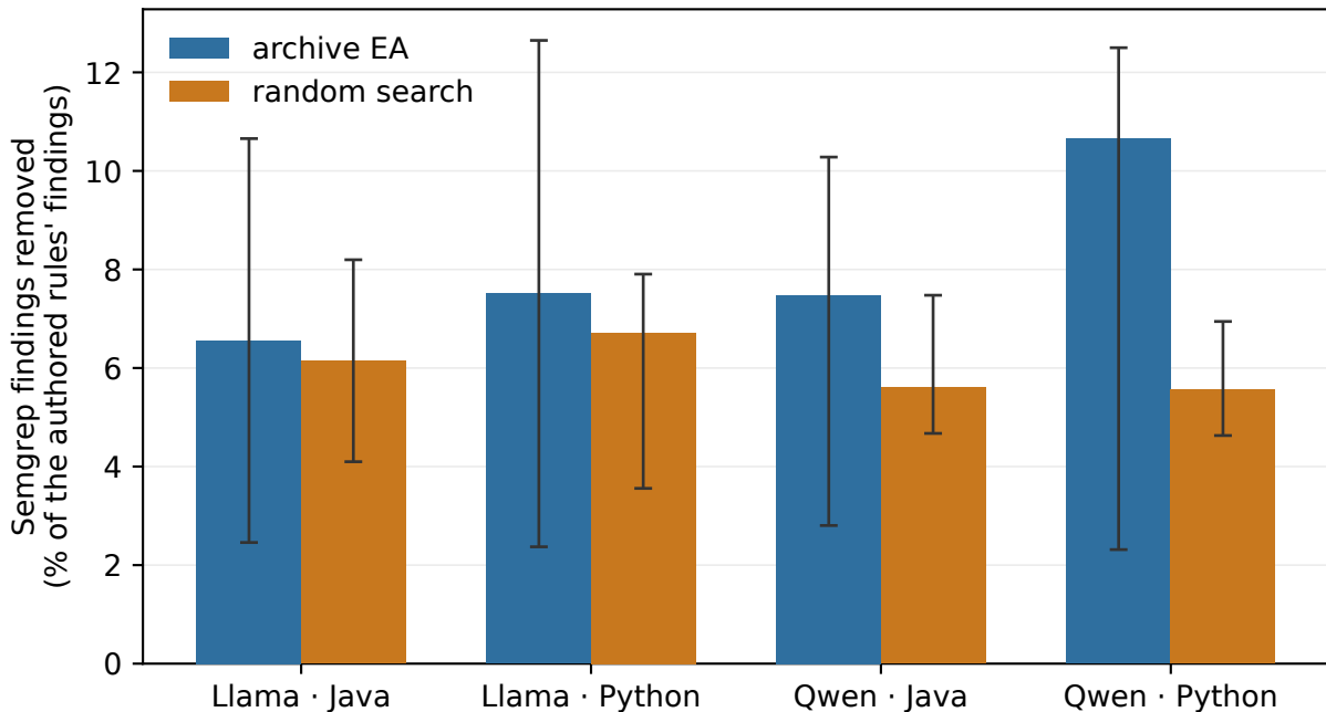
RQ1 — best structurally admissible rule-text/order mutations visited bar = median over seeds; whiskers = min-max
