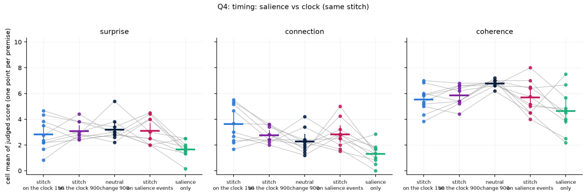
Figure 7: When to interrupt: the re-encounter stitch on the clock (150 and 900), the neutral change every 900, the stitch on salience events, and salience only (nothing injected). Post-interruption windows; one point per premise.
