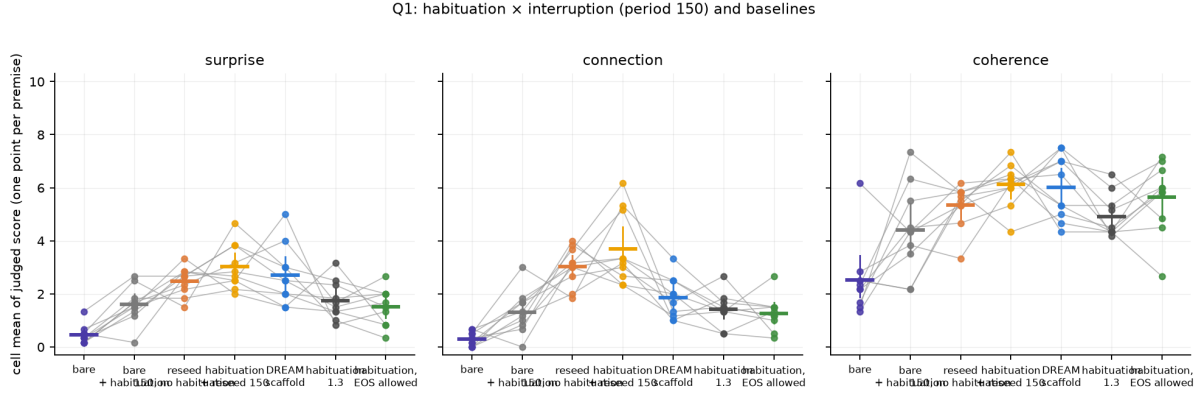
Figure 2: Habituation and interruption: bare, bare + habituation, interruption without habituation, habituation + interruption 150, the full scaffold, and the two habituation baselines (stronger penalty; EOS allowed). One point per premise, grey lines join the same premise across arms, bars are cell means with 95% bootstrap CIs over cells (Qwen3-30B-A3B, generated-only windows).
