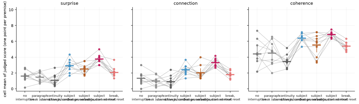
Figure 4: What carries the effect at period 300: no interruption, a paragraph break (sham), a continuity connective (sham), the subject change on the preserved context, the subject change without habituation, the subject change on a reset context, and a break on a reset context; one point per premise.
