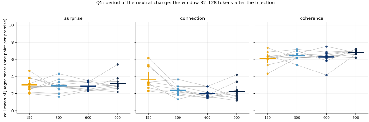
Figure 8: Period of the neutral change: the post-interruption window (32–128 generated tokens after the injection) at periods 150, 300, 600 and 900; one point per premise.
