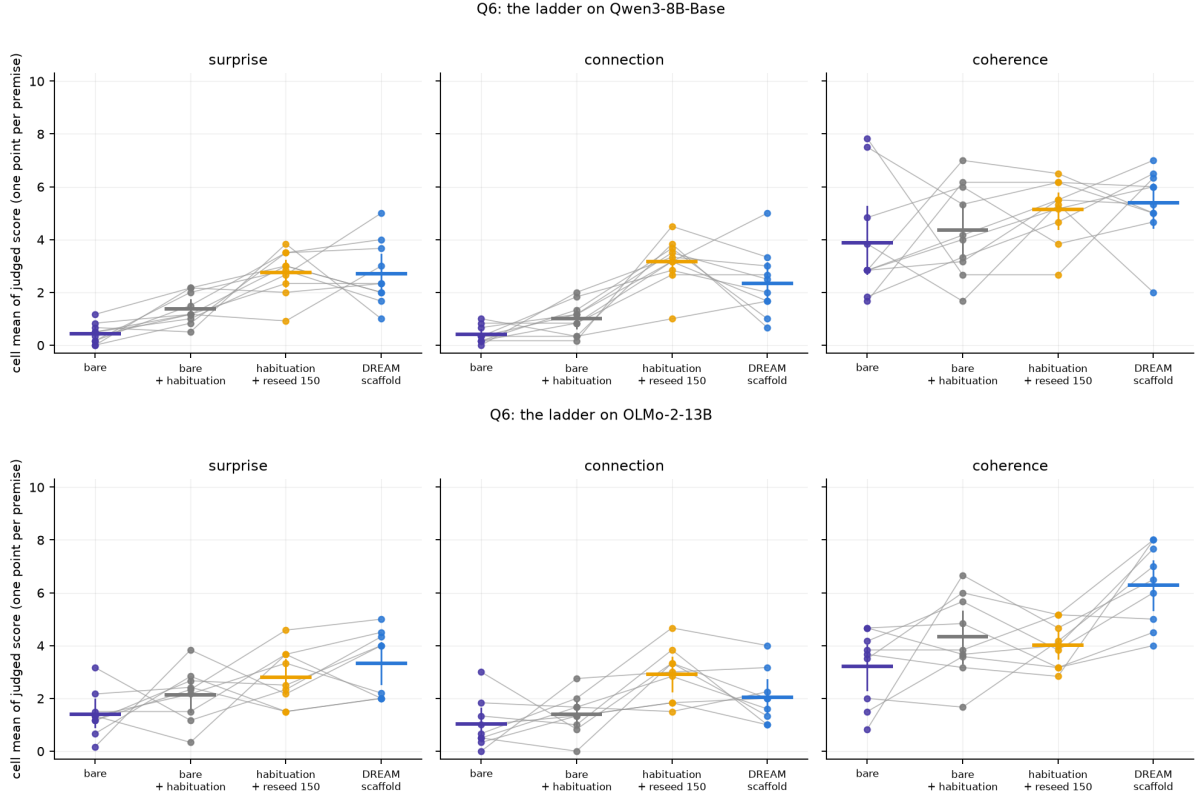
Figure 11: The ladder on Qwen3-8B-Base (top) and OLMo-2-13B (bottom); one point per premise.
