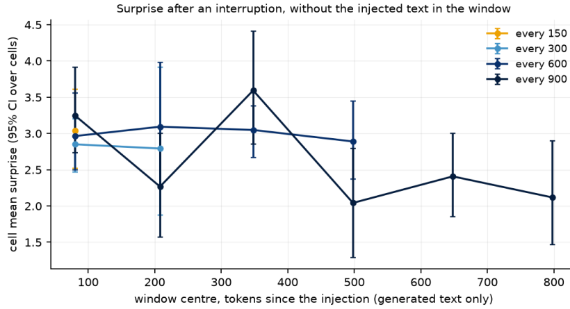
Figure 10: Decay: cell-mean surprise of generated-only windows by tokens since the injection, per period.
