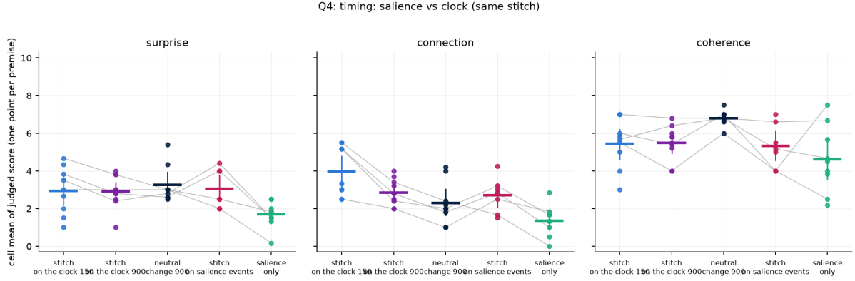
Figure 8: When to interrupt: the re-encounter stitch on the clock (150 and 900), the neutral change every 900, the stitch on salience events, and salience only (nothing injected). Post-interruption windows; one point per premise.
