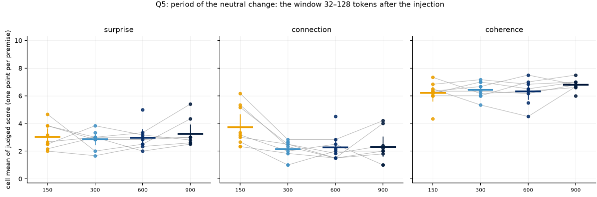
Figure 9: Period of the neutral change: the post-interruption window (32–128 generated tokens after the injection) at periods 150, 300, 600 and 900; one point per premise.
